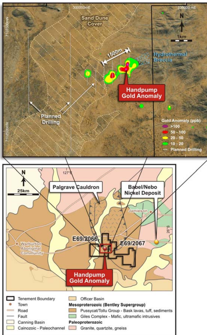
Figure 4. Handpump Gold Soil Anomaly
