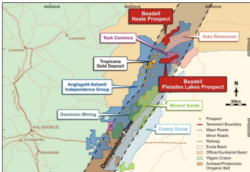
Figure 2 Tropicana East project location map
