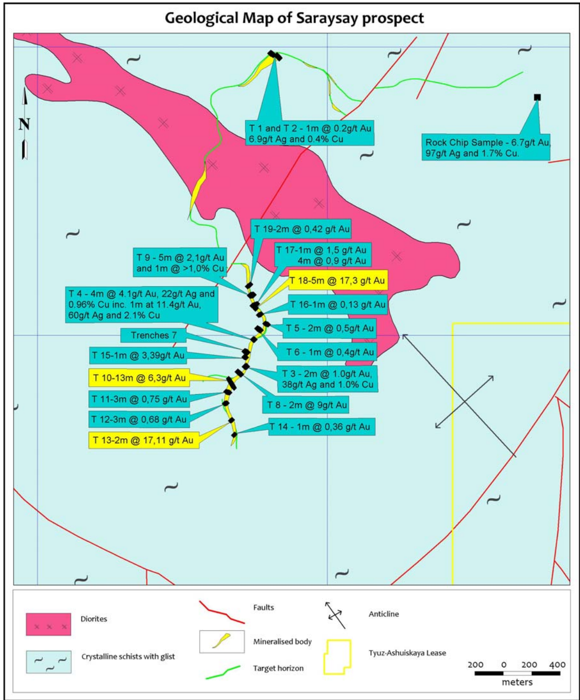
FIGURE 1 LOCATIONS AND RESULTS OF THE DRILLING AND TRENCH SAMPLING AT SARAYSAY
