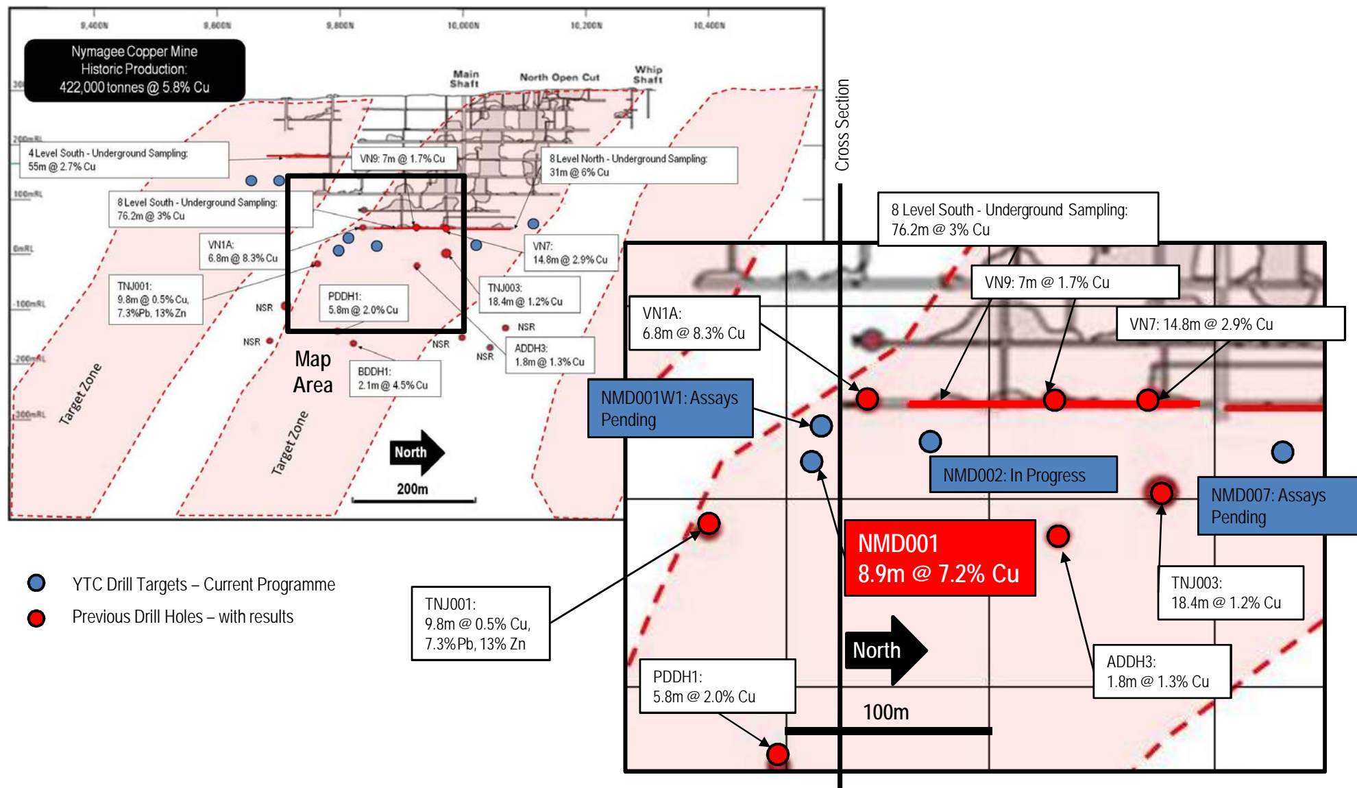
Nymagee Copper Mine – Long Section looking West
