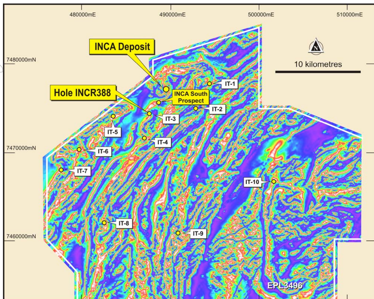
Figure 2: Regional TDR aeromagnetic image showing location of INCA-Type Targets within EPL 3496
