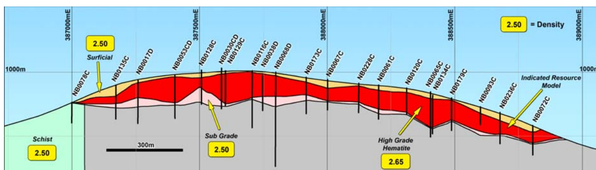
FIGURE 5: DRILLHOLE LOCATIONS AT NABEBA DEPOSIT
