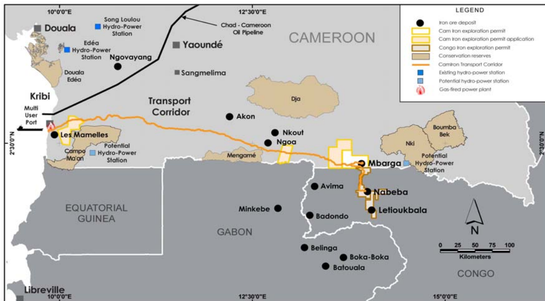
FIGURE 1: PROPOSED LOCATION OF PORT, TRANSPORT CORRIDOR AND MINES FOR THE MBALAM IRON ORE PROJECT
