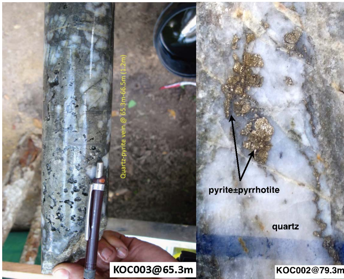
Fig.6: Kratie North, Target #2 – Drill core with massive pyrite quartz vein; quartz-pyrite-pyrrhotite vein
