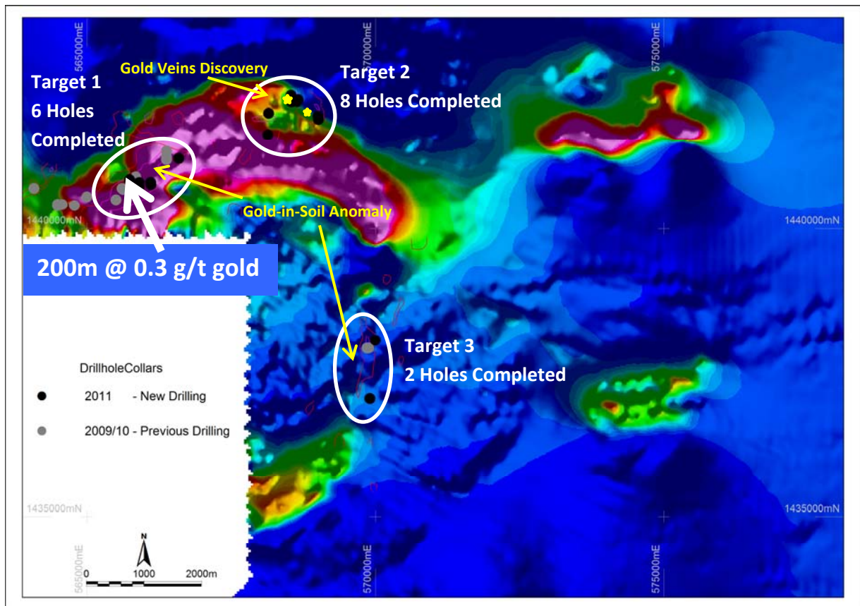
Figure 2: Kratie North Drill Targets overlain on Magnetic data.
