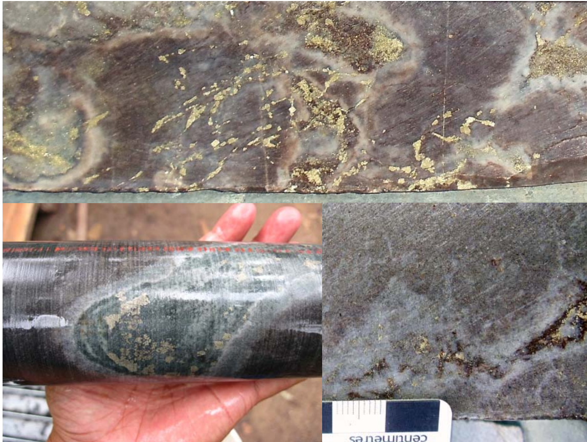
Fig.3: Kratie North, Target#1 - Drill core with quartz-pyrite-pyrrhotite veins (418m, 65m, 258m)
