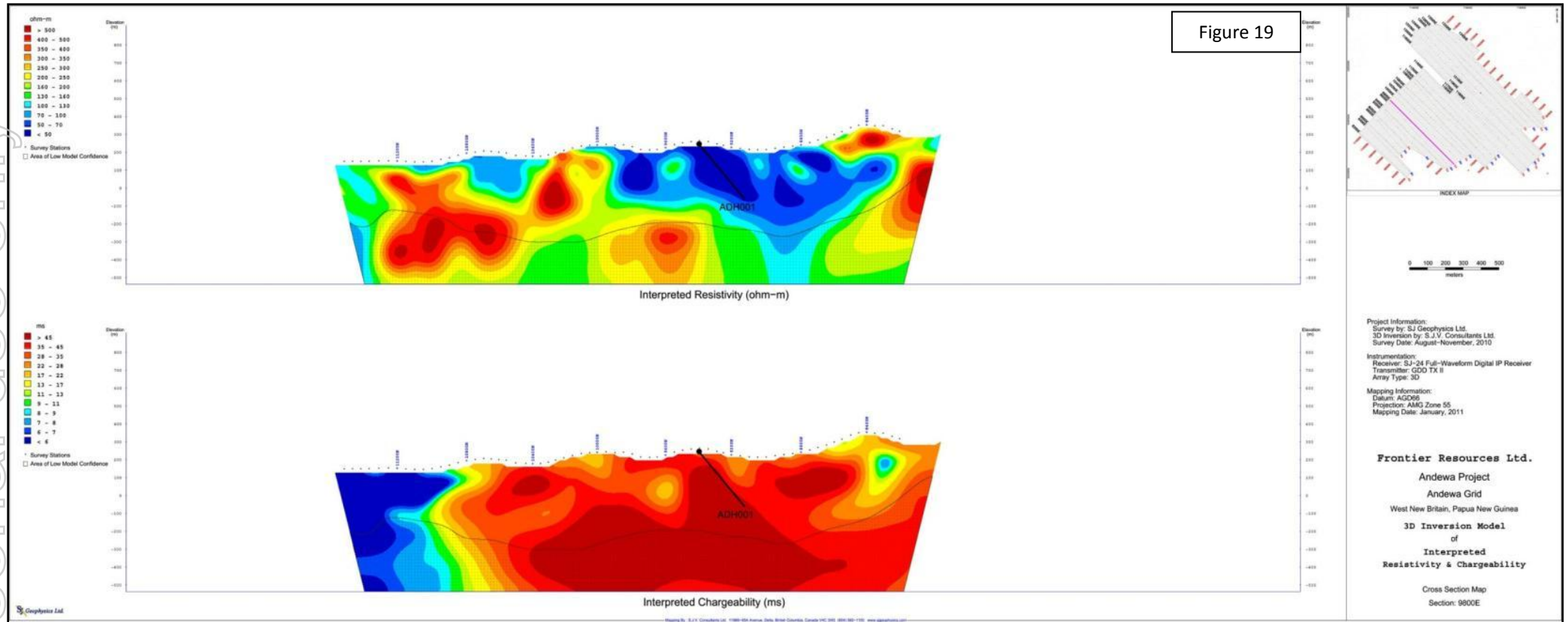
Figure 19. 3D-IP resistivity and chargeability cross section 9800E (geophysical /soil grid), showing drill hole trace ADH 001. Zones of strong conductivity correspond to the very low resistivity zones (dark blue). Additional holes are strongly warranted drilling both vertically into the bulk of the intense chargeability anomaly and also south into the strong conductivity (at depth).
