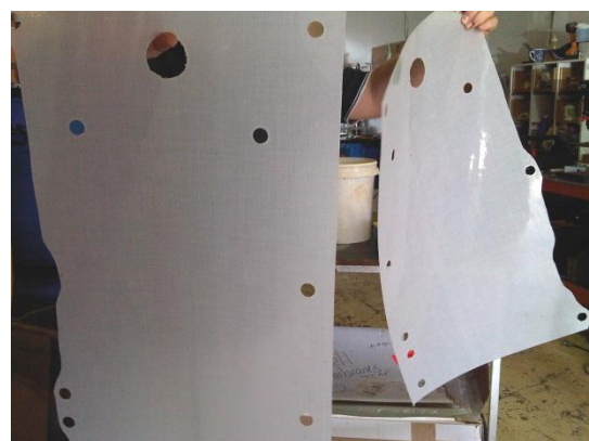
Figure 3 (left) – A close-up shot of the GE anion exchange membrane Figure 4 (right) – Membranes cut to size prior to being inserted into the pilot cell
