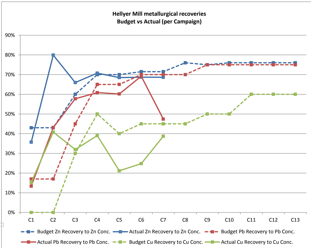
Figure 2: Planned and Actual recoveries for zinc, lead and copper to respective primary concentrates
