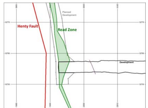
Read Zone plan view
