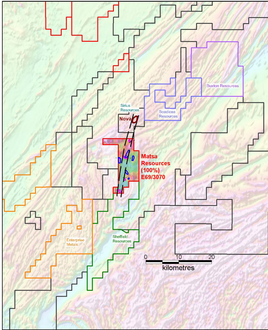
Figure 1: Symons Hill Tenement in the Fraser Range Region
