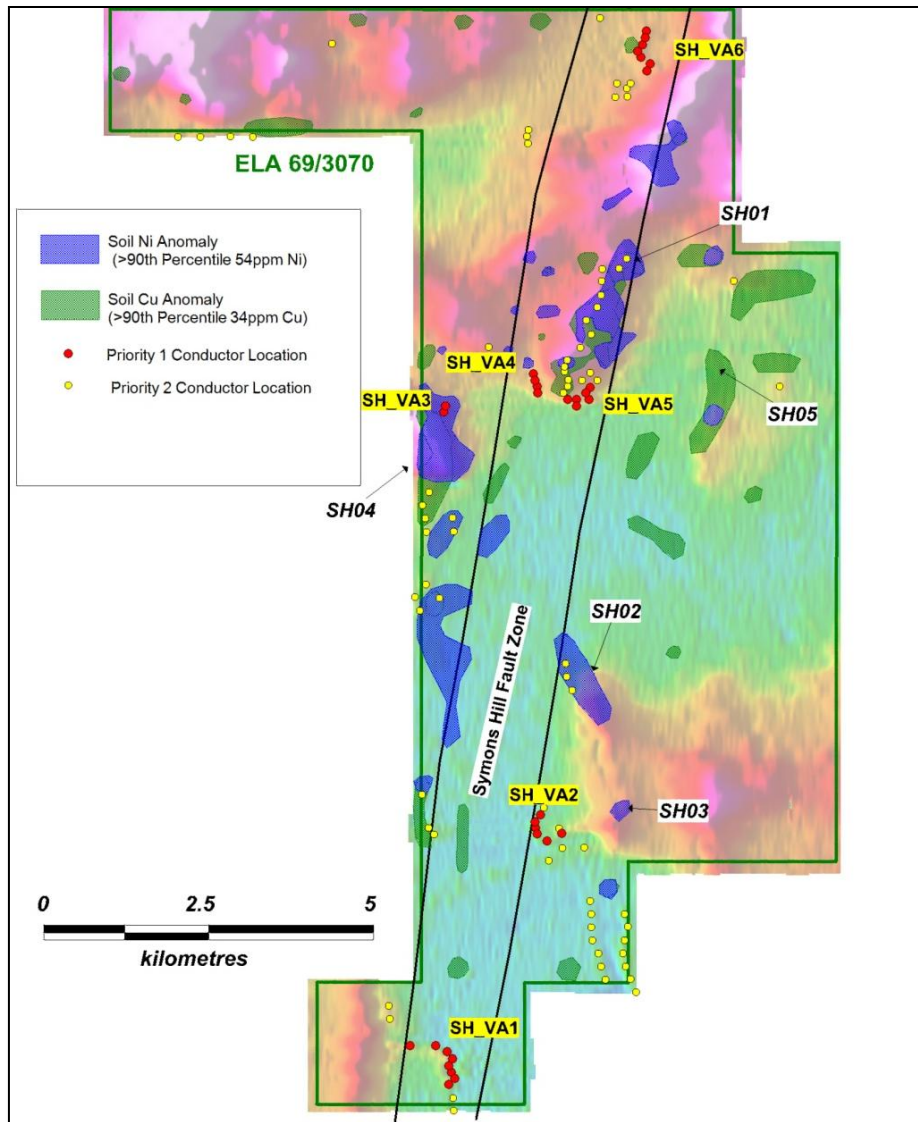
Figure 2: Symons Hill Tenement – VTEM Conductors and elevated Soils over VTEM Conductivity Image
