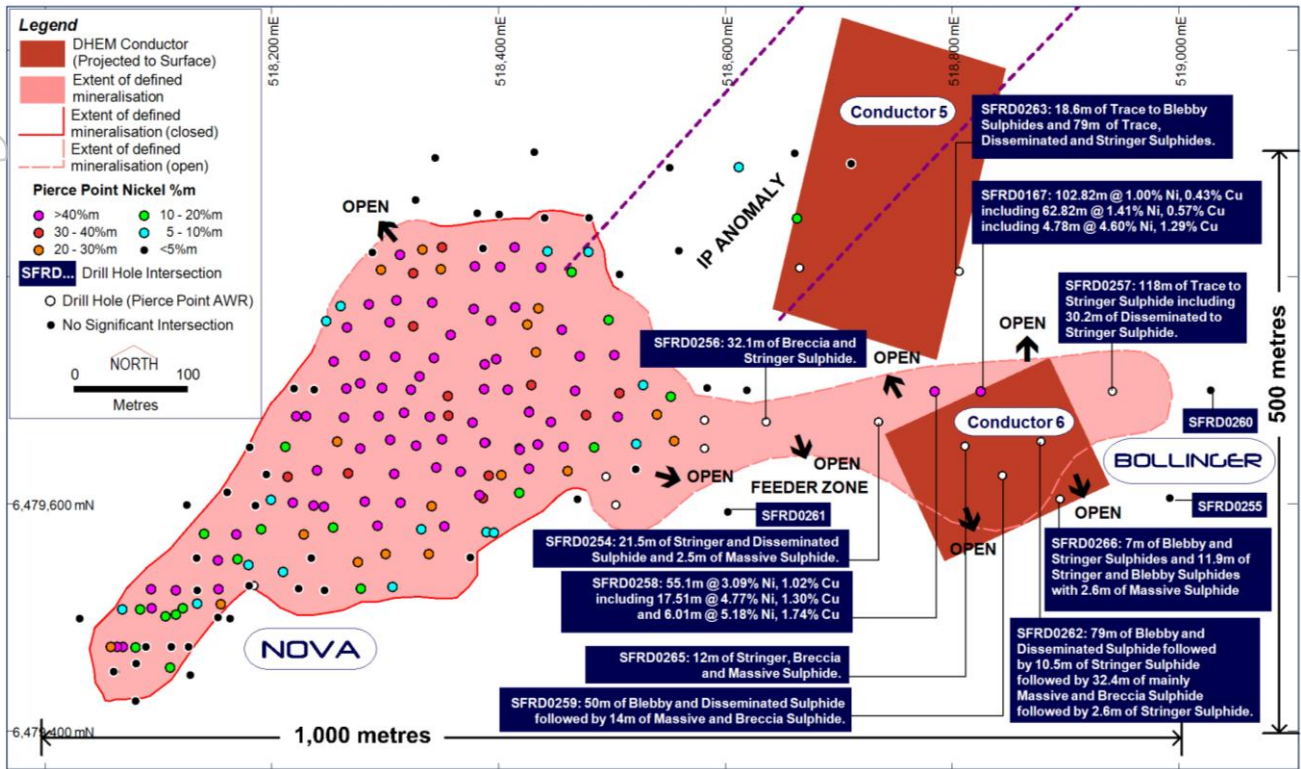
Figure 1. Plan projection showing new drilling at the Bollinger zone.
