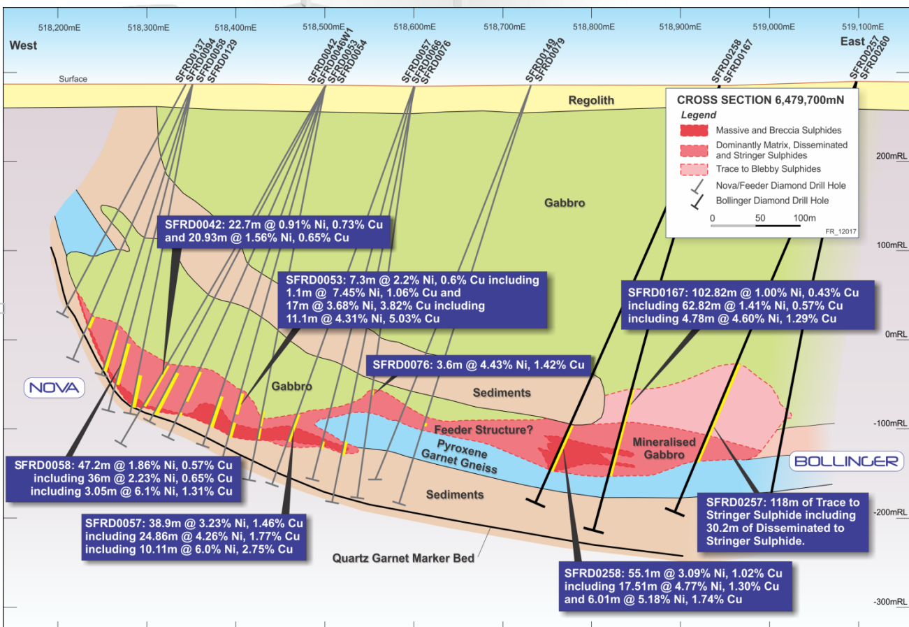
Figure 2. Cross section of line 700N showing new drill intersections in the Bollinger zone.
