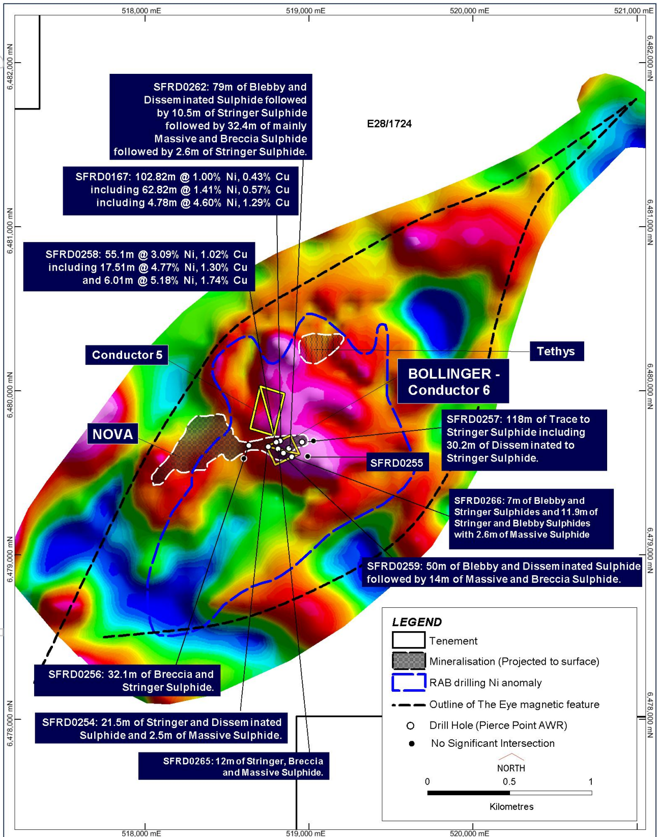
Figure 3. Gravity map of the Eye showing the location of the new drillholes at Bollinger in relation to conductors 5 and 6 and the large gravity anomaly in the centre of the Eye.
