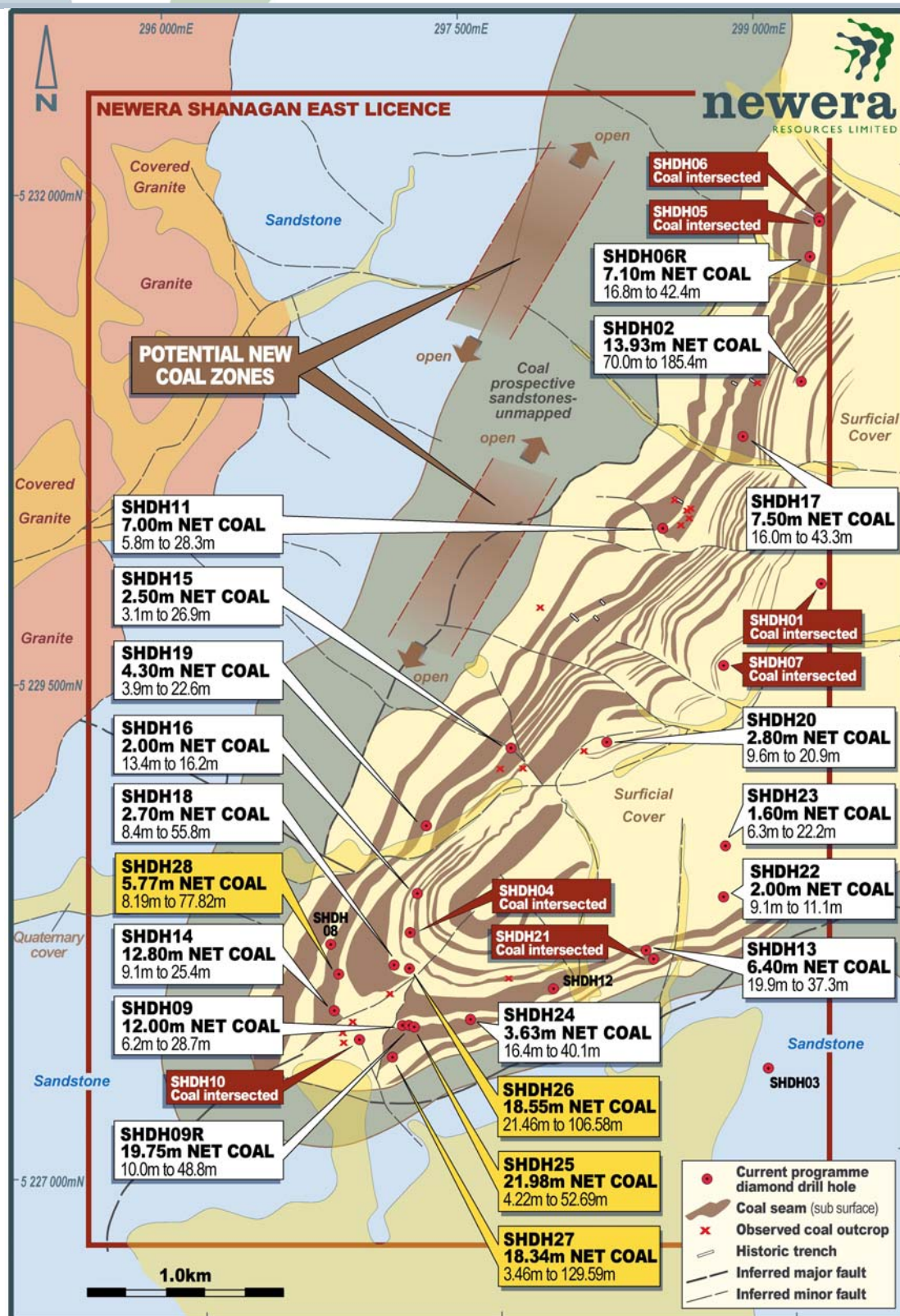
Figure 3: Previous drilling success and potential new coal zones outlined in the north of the Shanagan area.
