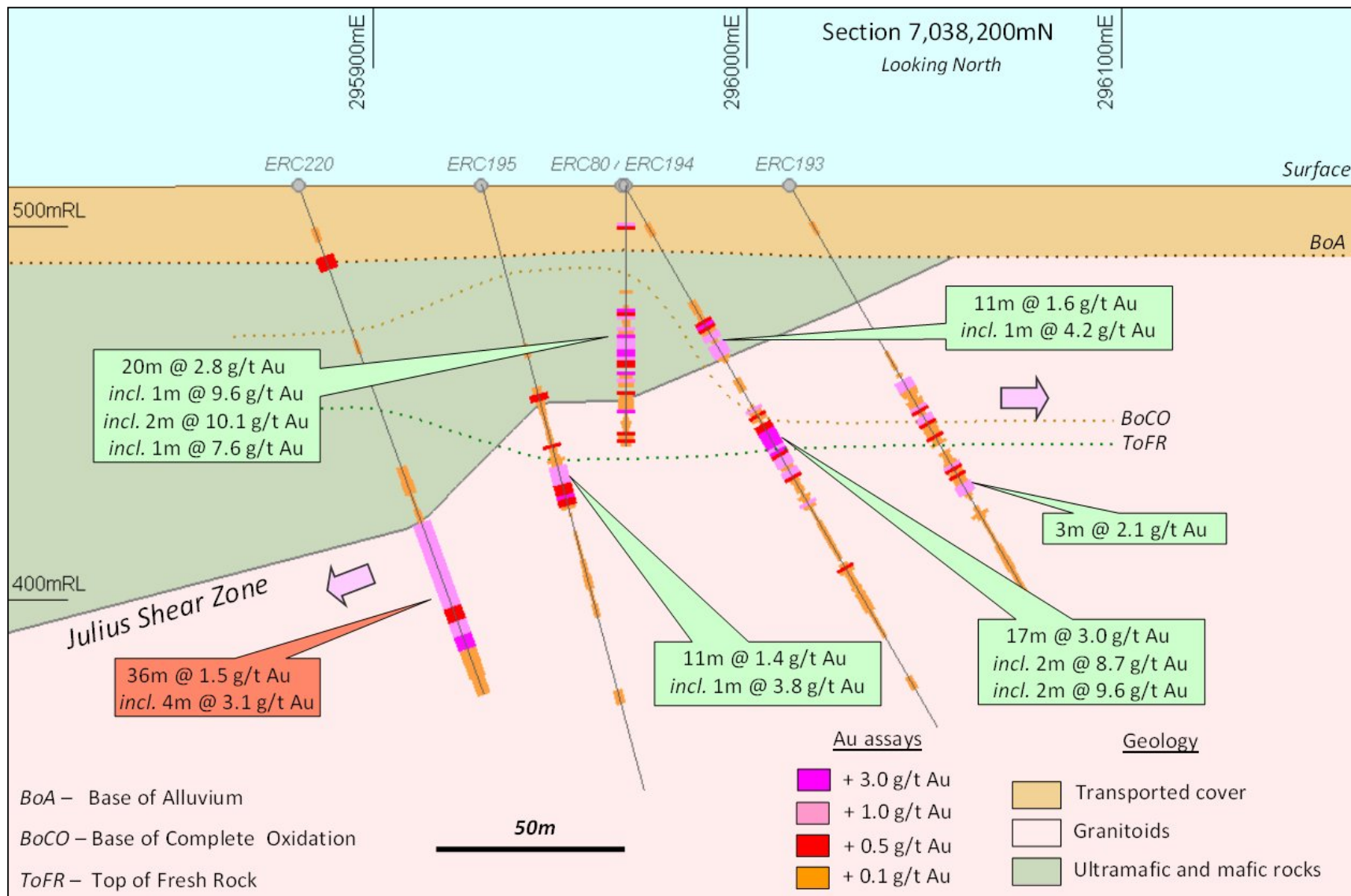
Fig. 8: Drilling results for drill hole ERC220.
