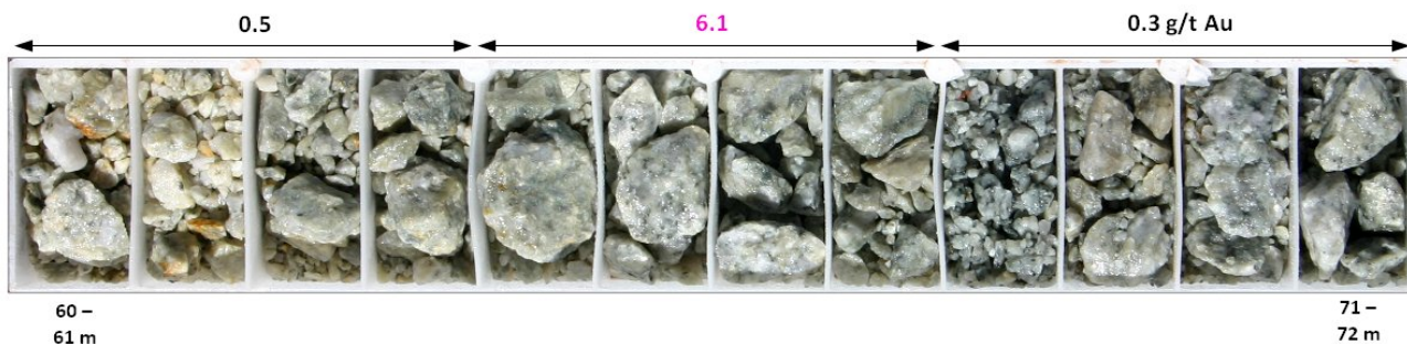
Fig. 9: Chip trays for ERC222 and ERC212.
