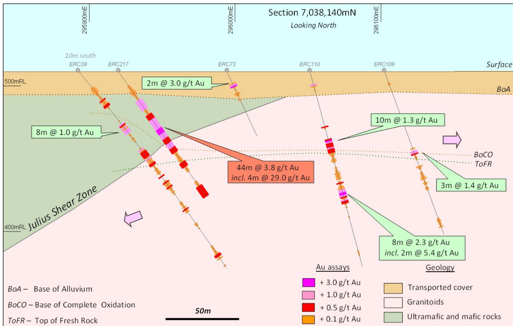
Fig. 5: Drilling results for drill hole ERC217.
