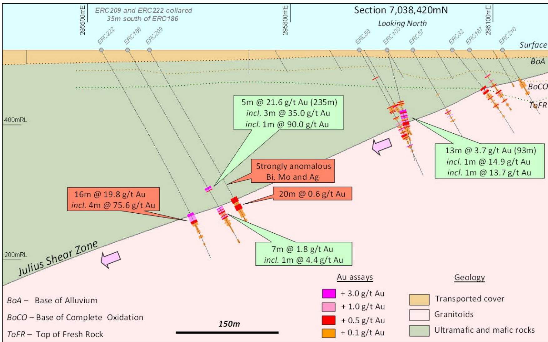
Fig. 4: Drilling results for step-out drill holes ERC186, ERC209 and ERC222.
