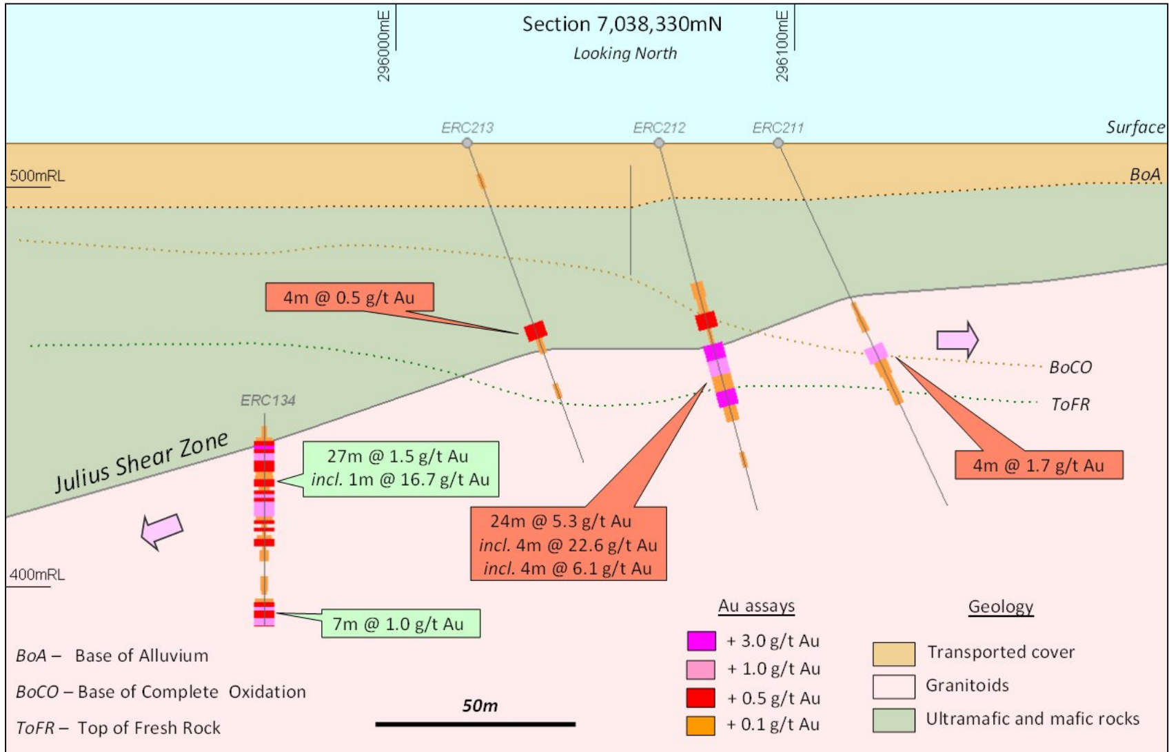
Fig. 6: Drilling results for drill holes ERC211, ERC212 and ERC213.
