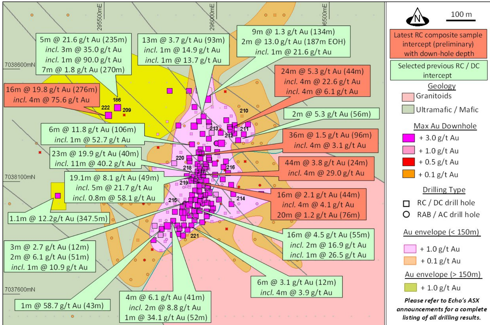
Fig. 3: Summary of drill intersections.
