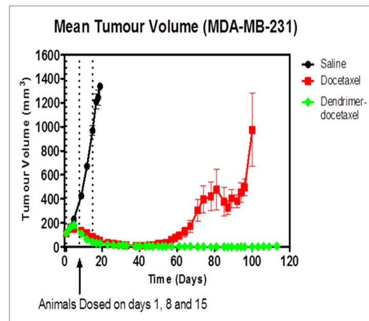
Saline Control 19d
