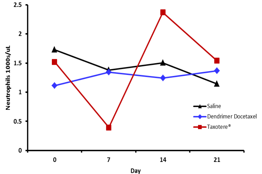
DEP™ Docetaxel formulation and Taxotere® at equivalent doses (based on docetaxel; 9mg/kg); n=6 rats/group
