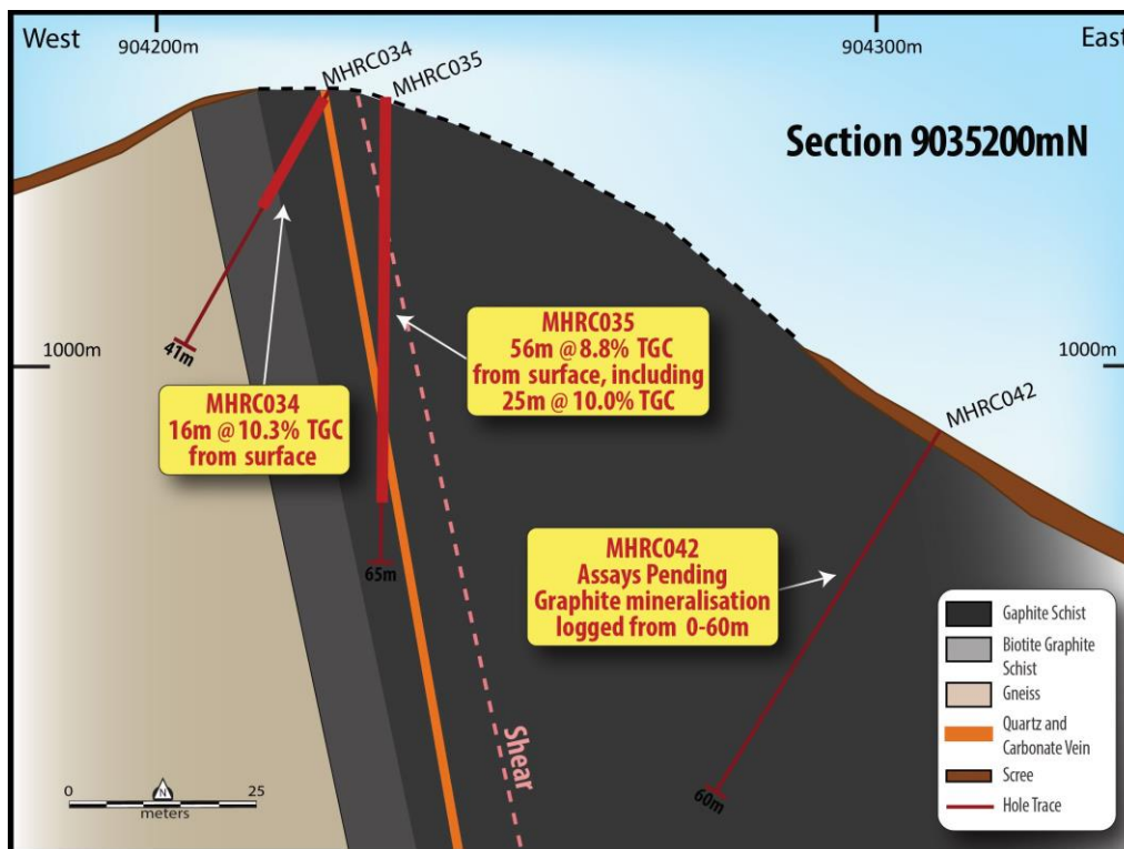
Figure 1 – Geological Interpretation of section 9035200 mN
