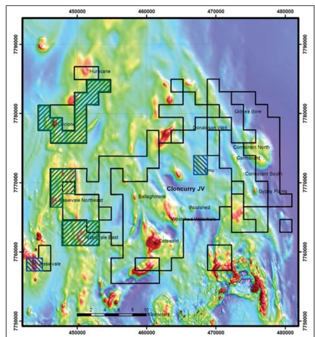
Figure 10: Planned magnetic surveys (blue shading), gravity surveys (green shading) with respect to regional magnetic image for the Cloncurry JV.
