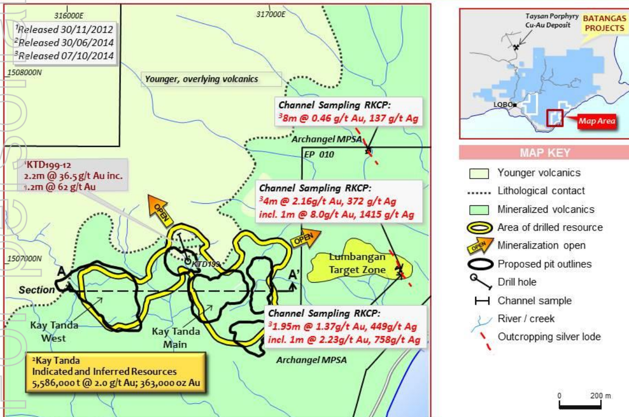
Figure 1: Archangel Prospect plan, with location of Lumbangan rock chip channel sampling results
