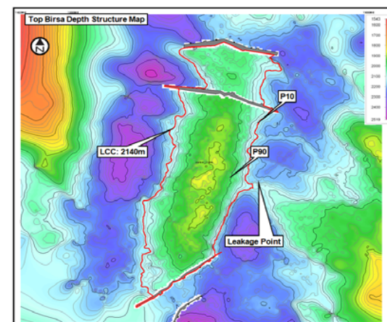
Top Birsa Depth ISIS – CPR 2013
