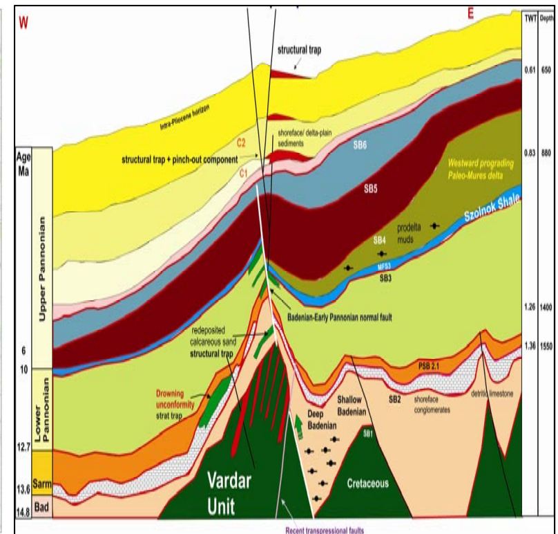
Cross Section Highlighting Potential Oil and Gas Targets
