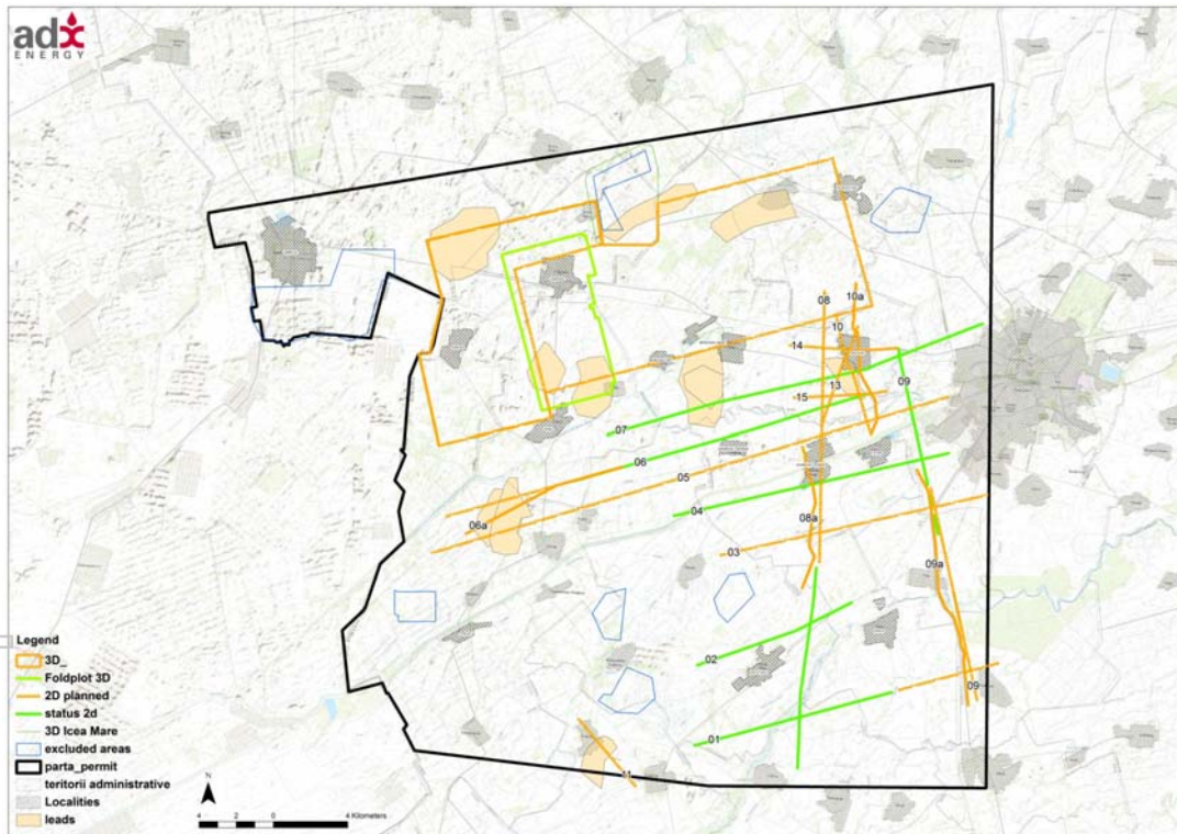
Parta Permit 2D and 3D Planned Seismic Program
