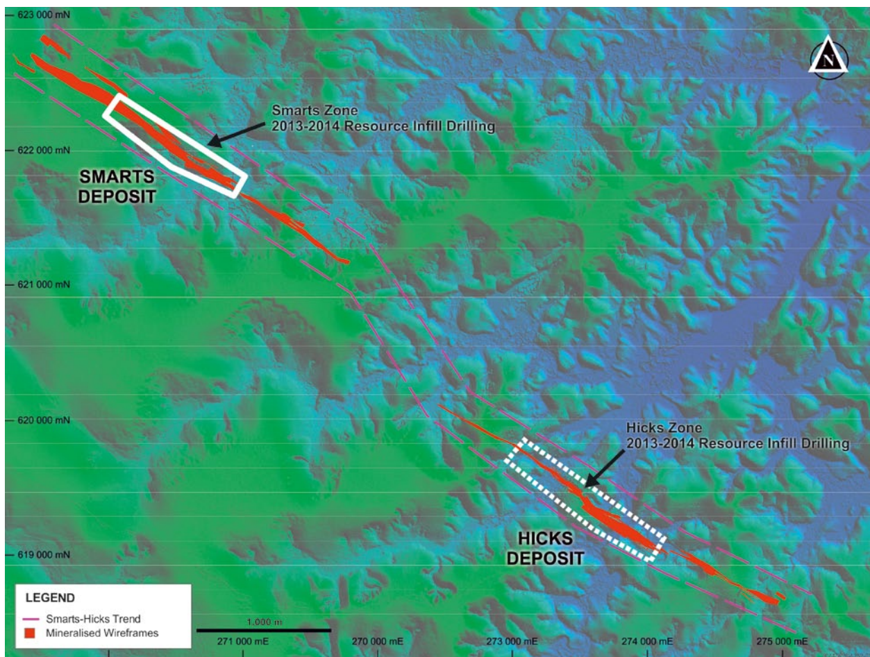
Location Plan of Smarts and Hicks Deposits on Digital Terrain Model
