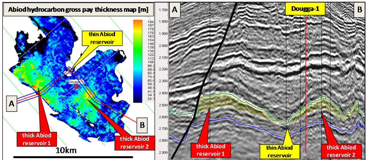
Figure 1: 3D seismic section through the Dougga gas condensate discovery. The Dougga-1 discovery is not optimally placed neither with respect to the structural location (300 meters downdip) nor the sweet spot zones of thick and most likely best Abiod reservoir development. The hydrocarbon gross pay map shows that Dougga-1 intersected about 70 meters of Abiod gross reservoir, whereas several areas with up to 200 meters of gross Abiod reservoir can be expected based on the high resolution 3D seismic evidence (green, yellow colors).
