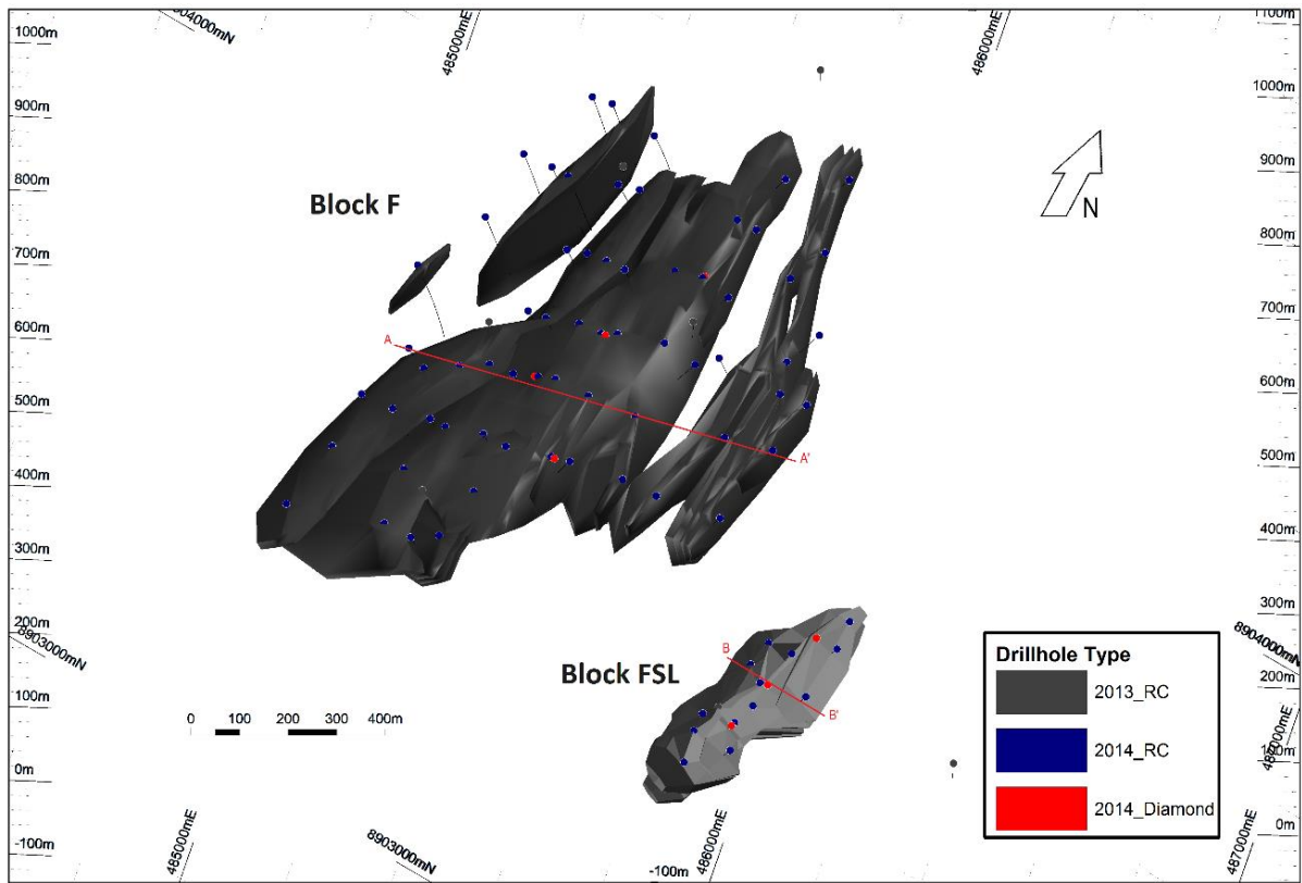
Figure 3: Block F deposits F and FSL (F South) with corresponding section lines.
