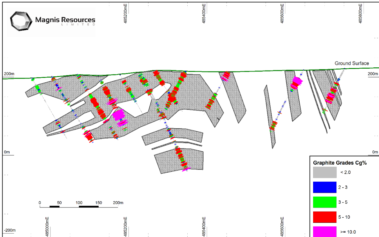
Figure 4: Cross section A-A' looking North within Block F, showing modelled mineralisation with downhole grades highlighted.
