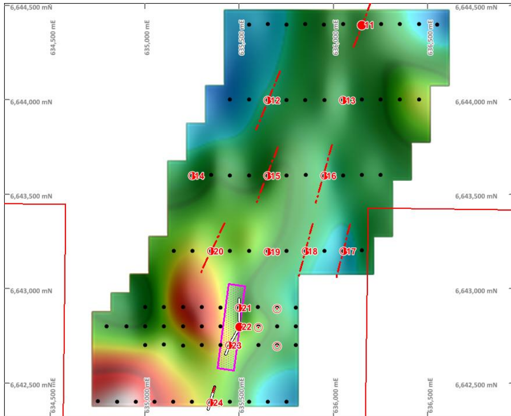
Figure 4: Fraser Range North 2014 MLTEM survey; central block. Interpreted anomalies (red circles) and possible conductor axes (red / white lines) overlain on late time channel (channel 35, 156mS) EM amplitude image. The purple polygon is the best fit modelled conductive plate
