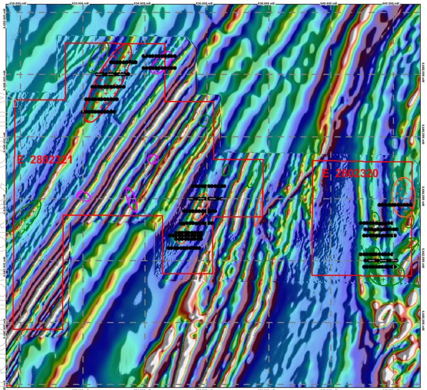
Figure 6: Fraser Range North 2014 MLTEM survey line locations (black dots). Overlain on FVD RTP magnetics, with interpreted intrusive locations and Ram tenement outlines
