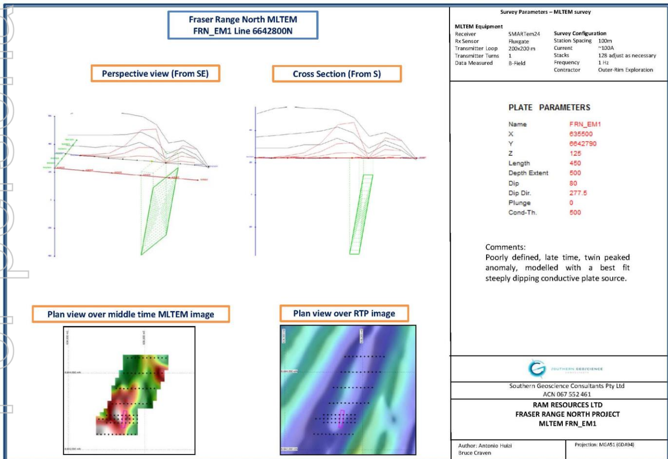
Figure 5: Modelling Summary, FRN-22 MLTEM anomaly
