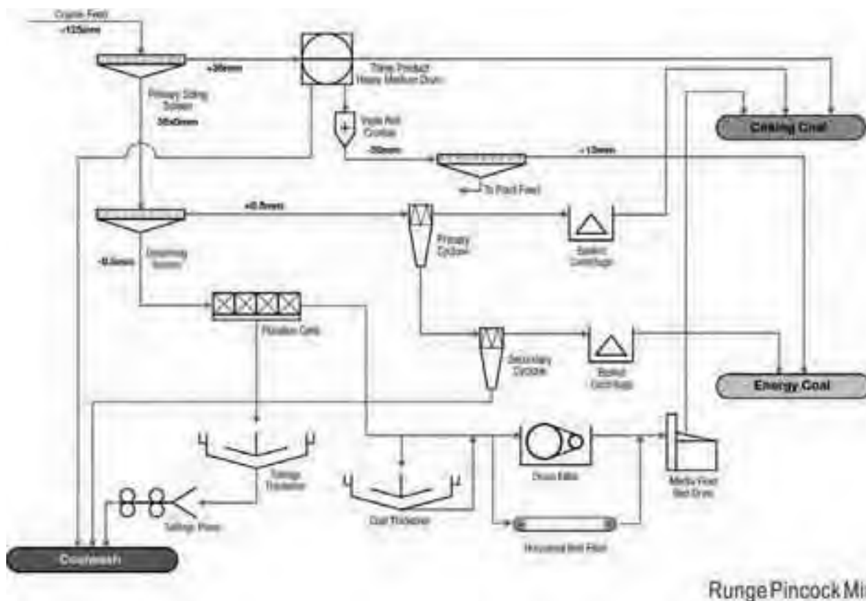
Figure 9-2 - Dendrobium Coal Handling and Processing Plant Flow Sheet
