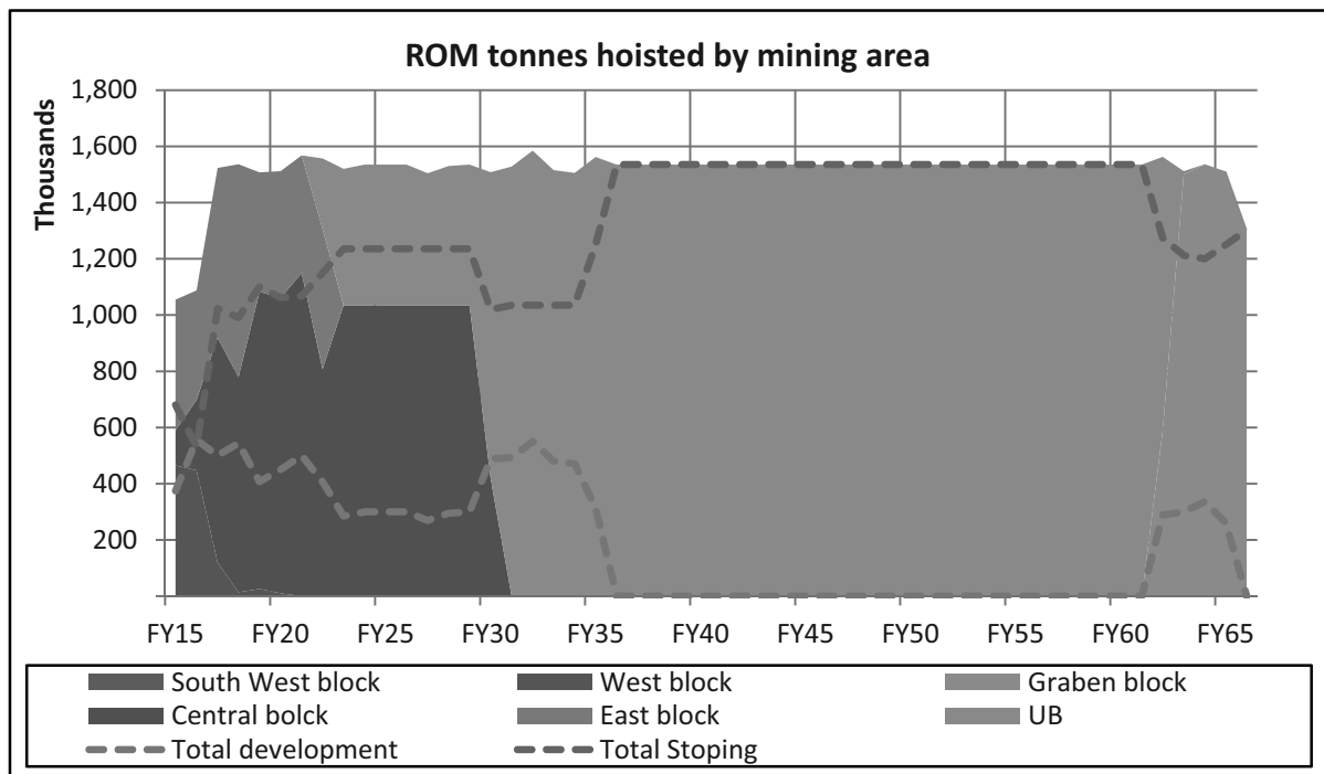
Figure 34 FY15 LoA plan showing tonnes hoisted by mining area
