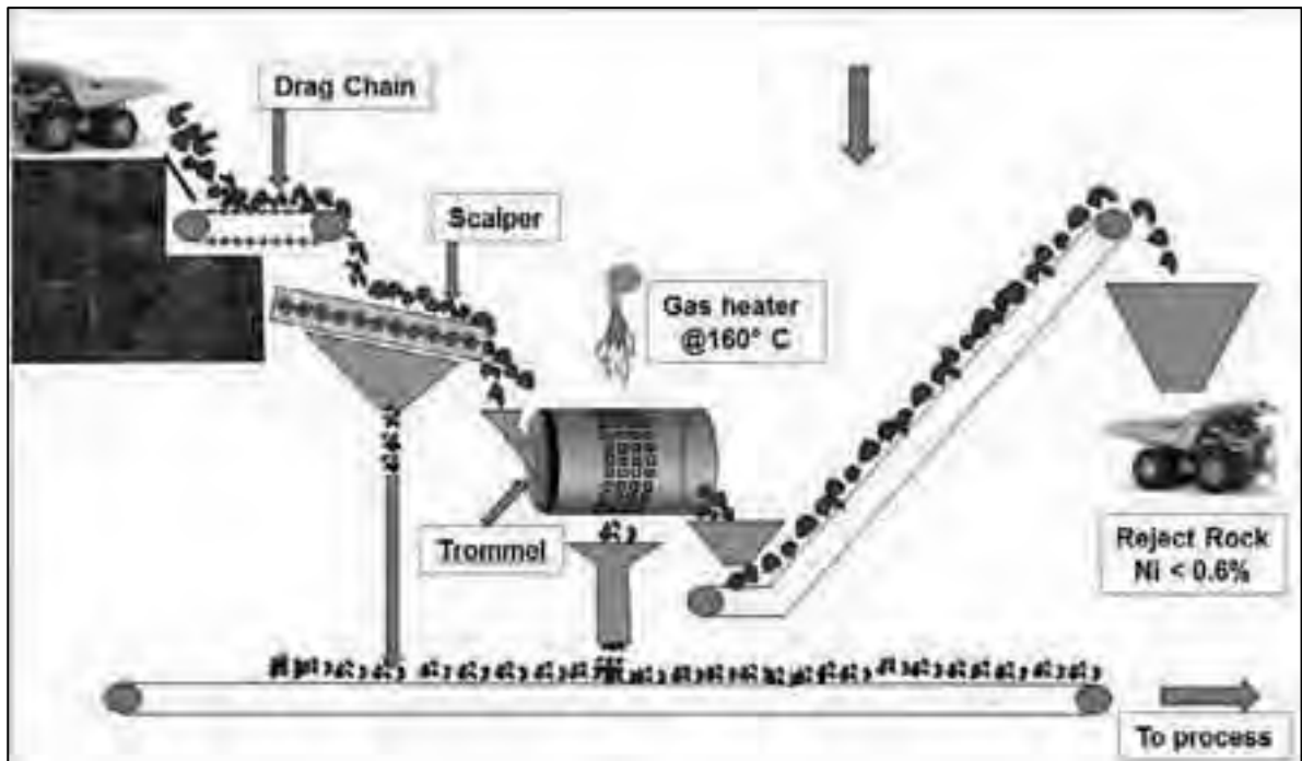
Figure 8-7: Simplified flowsheet of pilot plant under construction for testing in December Source: CMSA (2014)
