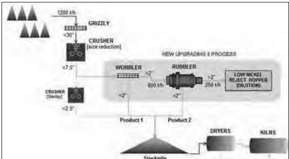
Figure 8-8: Flowsheet of proposed Upgrade 2 plant Source: CMSA (2014)
