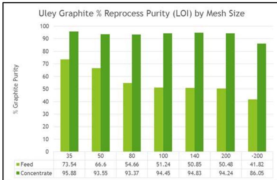
Figure 1. Additional Grinding Test % Loss on Ignition (LOI) Purity Results by Mesh size (Uley Graphite™ plant) 29 August 2015
