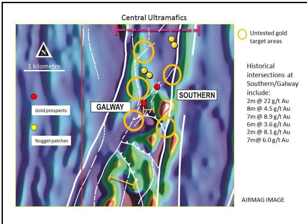
FIG 3. A and B - Position of gold target areas surrounding Galway – Southern prospects
