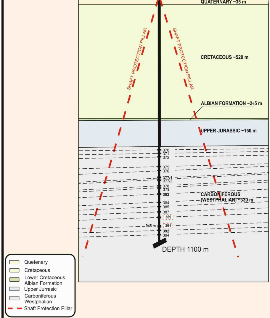
Figure 14: Lublin Coal Project - Shaft Design Concept
