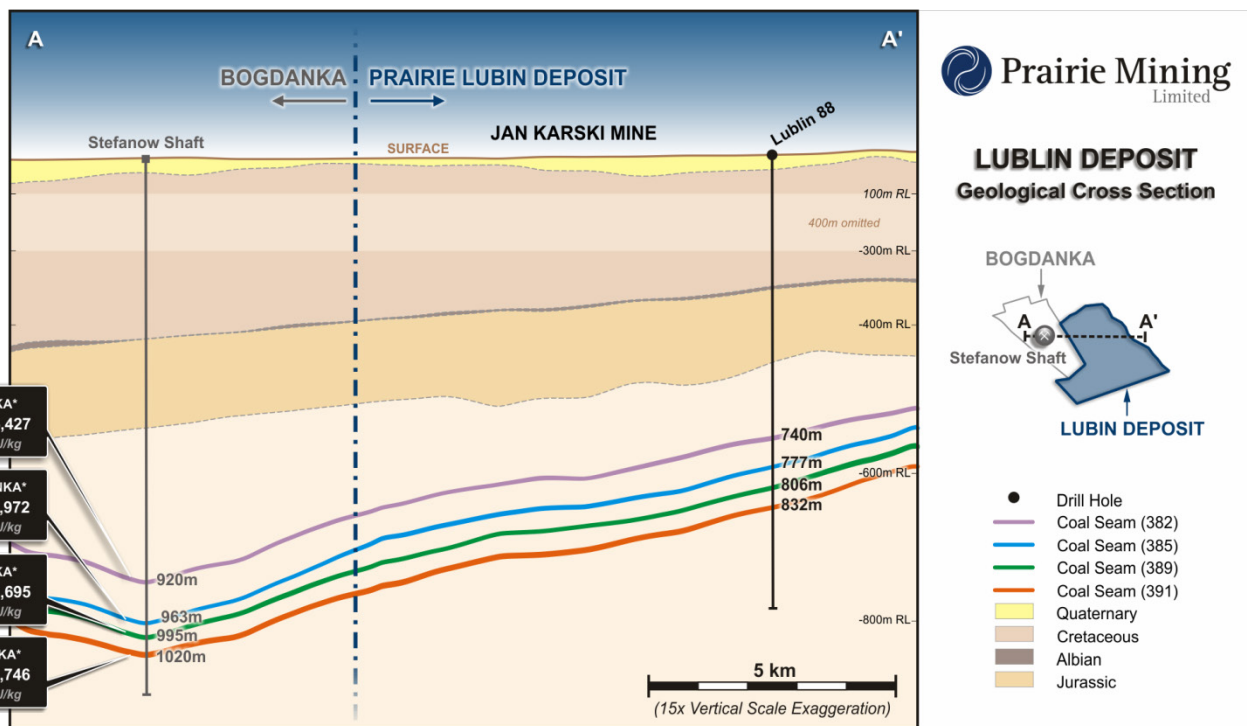
Figure 13: LCP – Geological Cross Section
