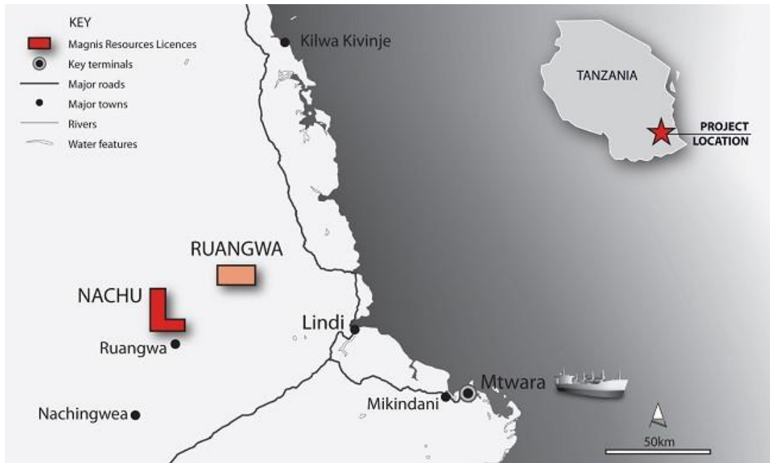
Figure 1: Location of the Nachu Graphite Project depicting proximity to the port of Mtwara
