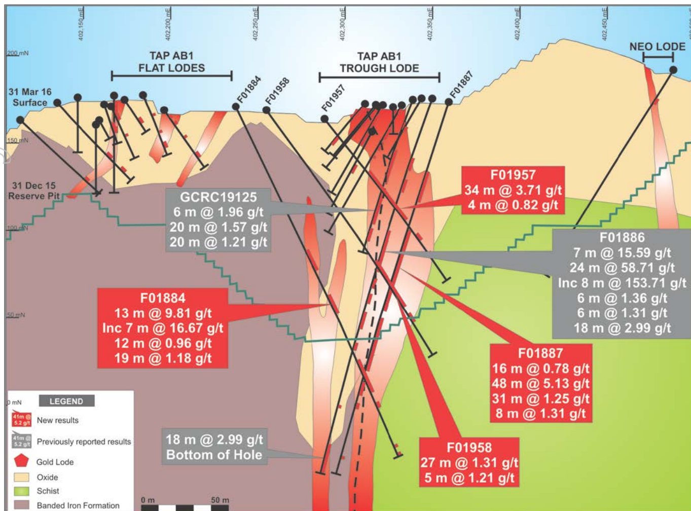
Figure 3. Tap AB1 Trough Lode cross section 93825N looking north.
