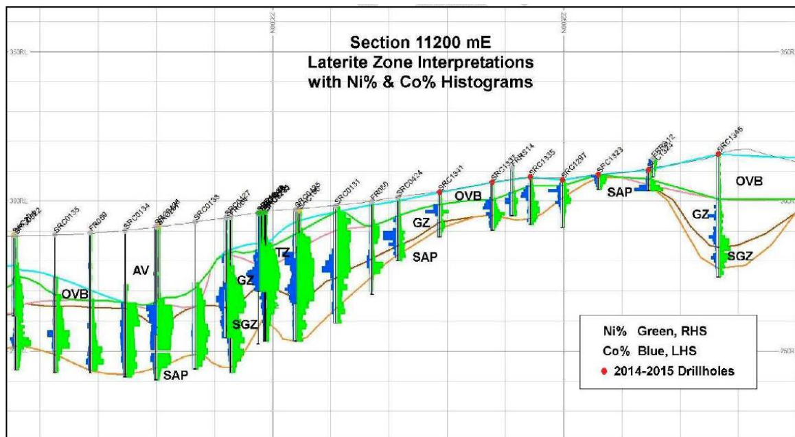
Figure 17: Section 11200mE Laterite Zone Interpretations (vertical exaggeration = 5:1)
