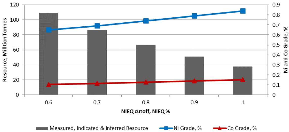
Figure 11: Contained nickel and cobalt resource and grade for a range of cut-off grades
