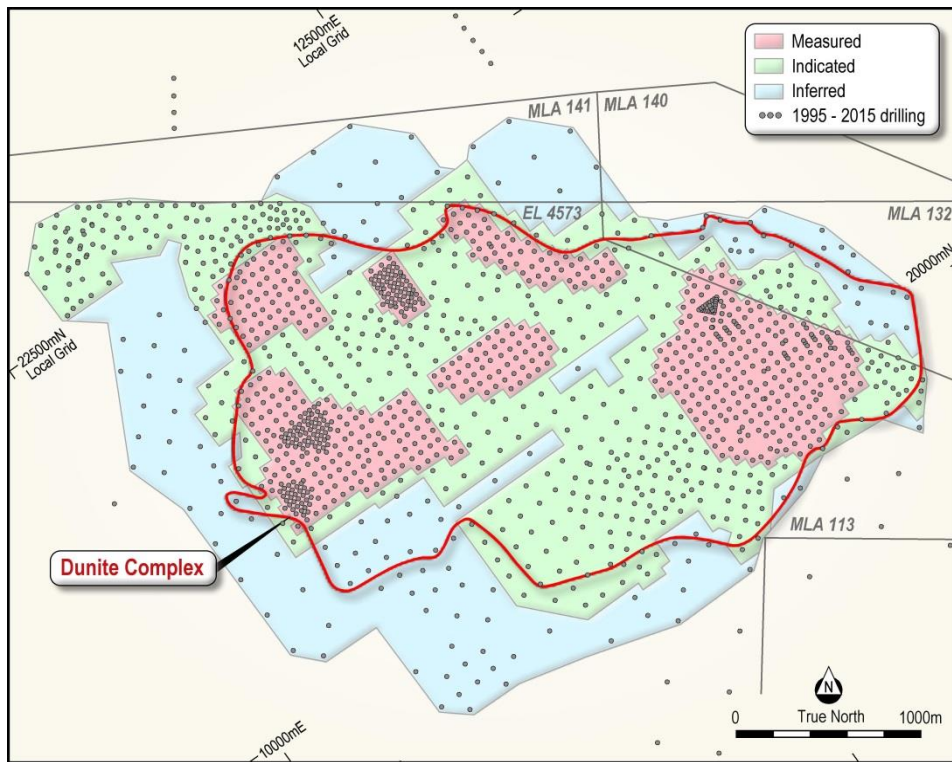
Figure 12: Syerston Cobalt/Nickel Mineral Resource Area
