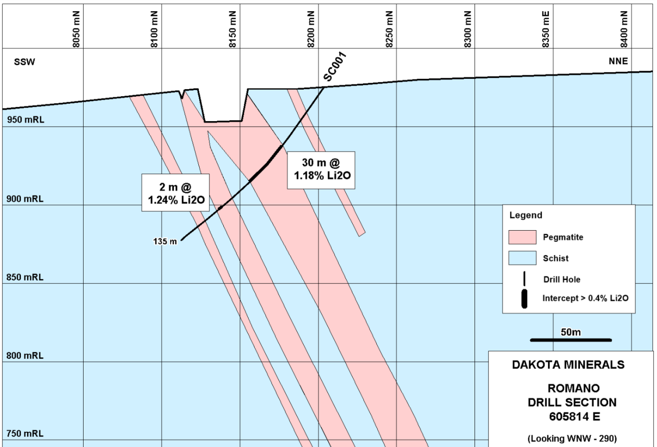
Figure 4: Drill sections from Romano pegmatite, Sepeda Project, showing results received to date, and logged geology.
