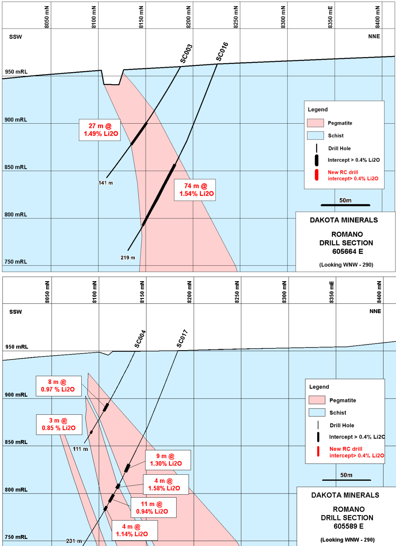
Figure 3: Selection of drill sections from Sepeda (Romano Pegmatite), showing logged geology and latest results.
