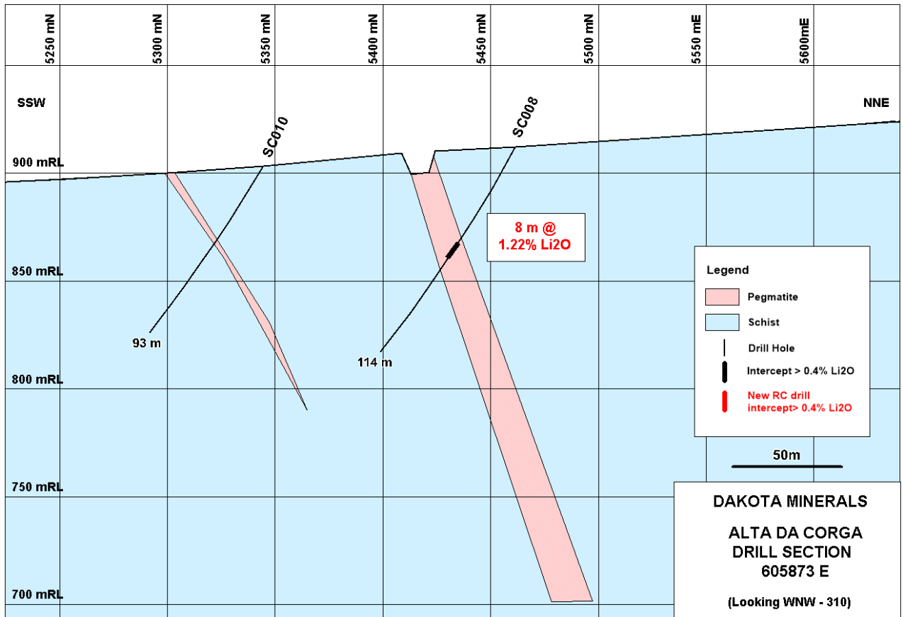
Figure 5: Selection of drill sections from Sepeda (Alto da Corga pegmatite), showing logged geology and latest results.
