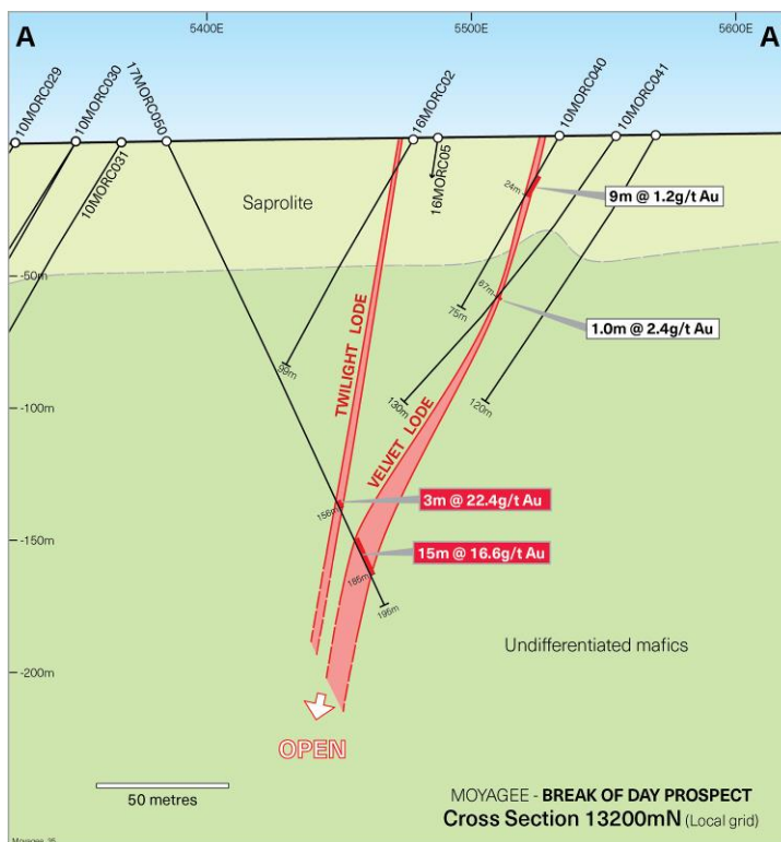
Figure 2: Break of Day cross section 13200mN – local grid (vertical section through mineralisation)
