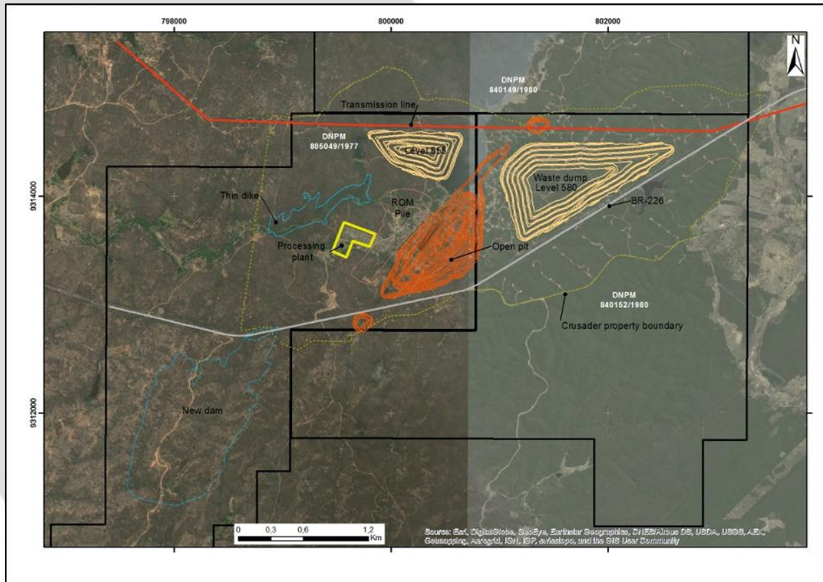
Figure 6: Borborema General Layout 2016, Stage 1
