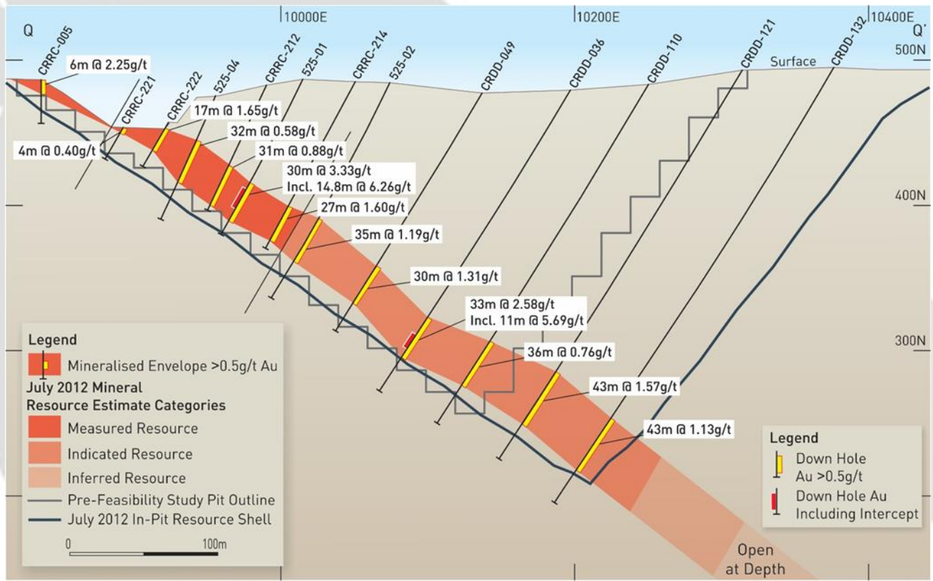
Figure 4: Borborema Gold Project, sample Cross Section Q-Q'
