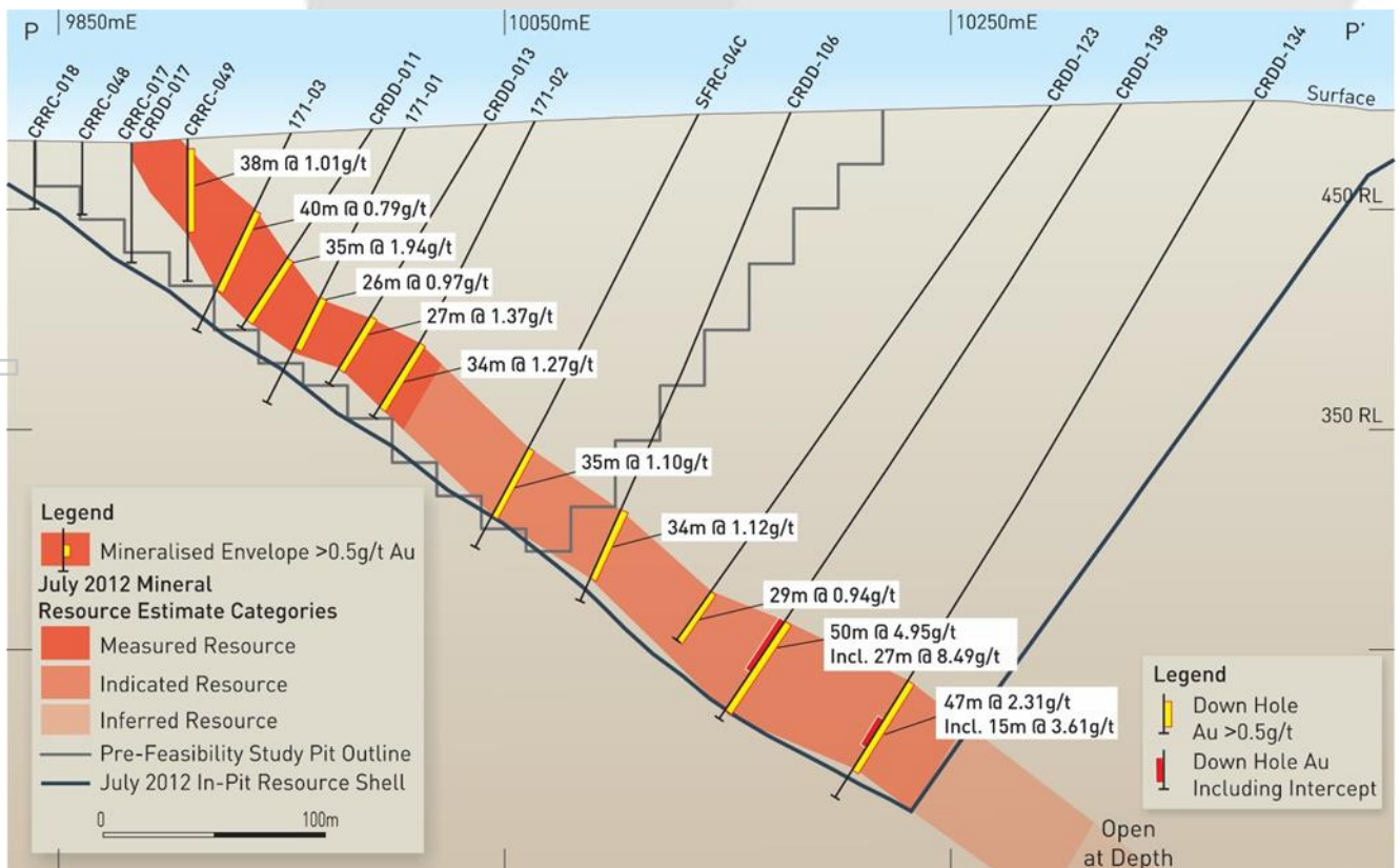
Figure 3: Borborema Gold Project, sample Cross Section P-P'
