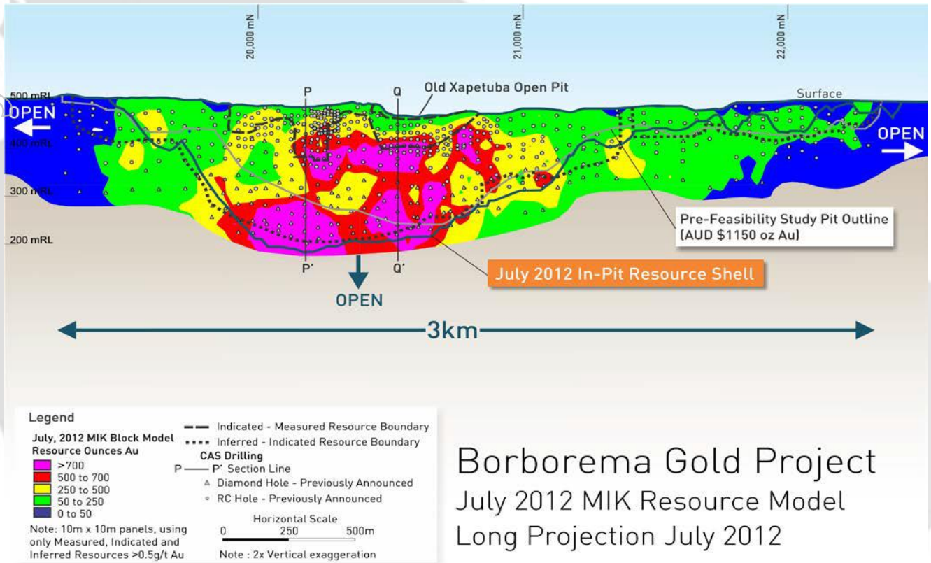
Figure 2 Long Section for the Borborema Gold Project (as per ASX release of 26 July 2012)
