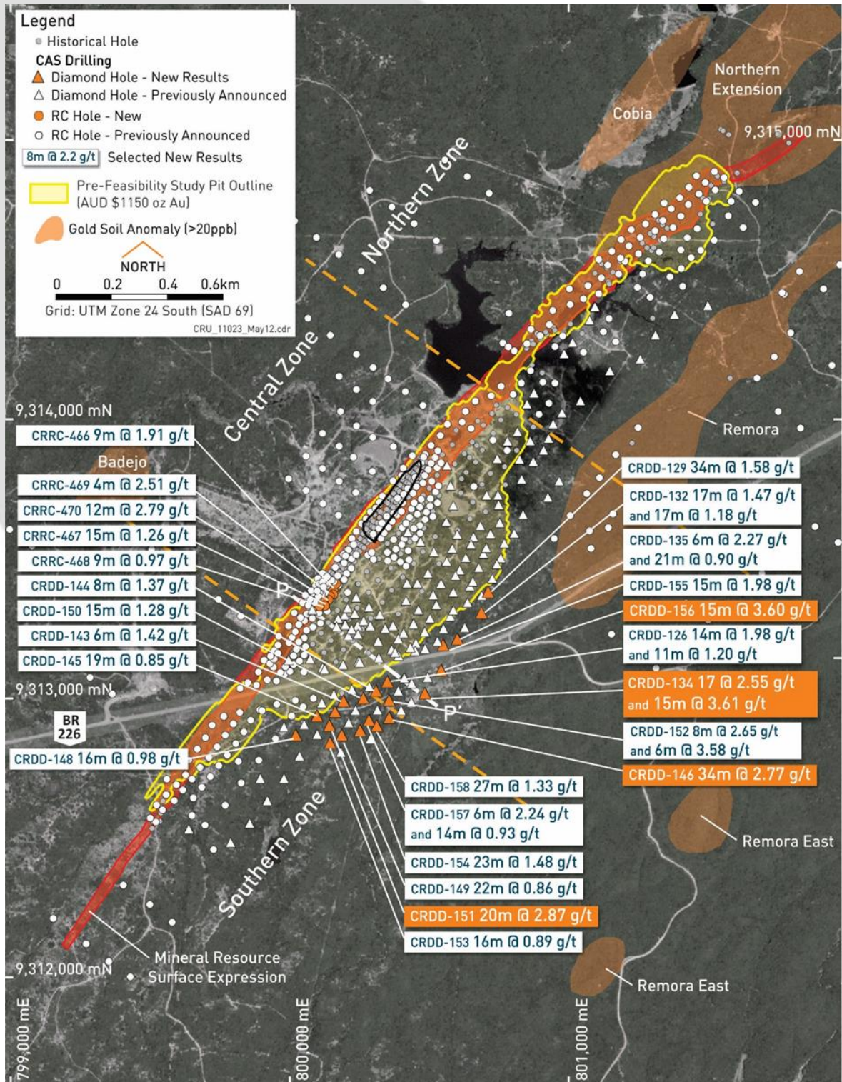
Figure 1: Drillhole Location Plan for the Borborema Gold Project (as per ASX release of 6 June 2012)
