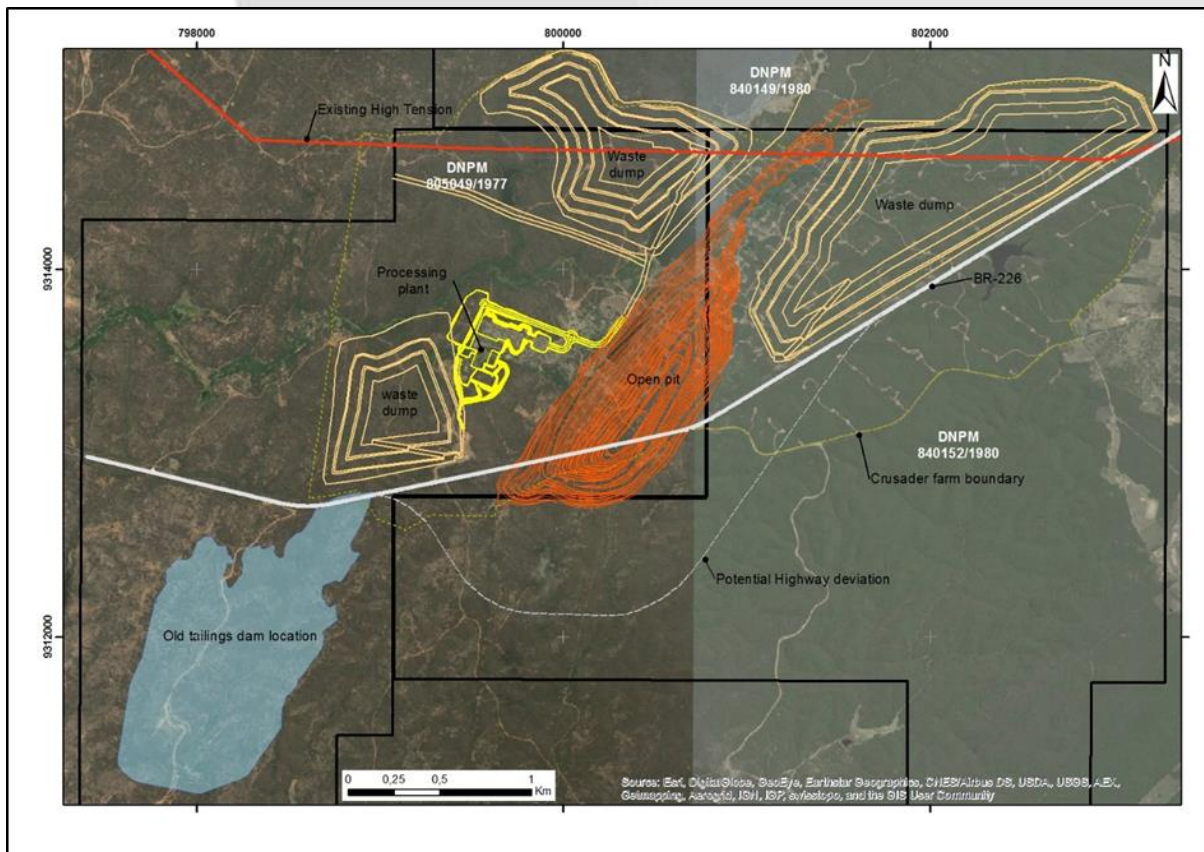
Figure 5: Borborema General Layout – 2013 – Showing Ore Reserve Open Pit
