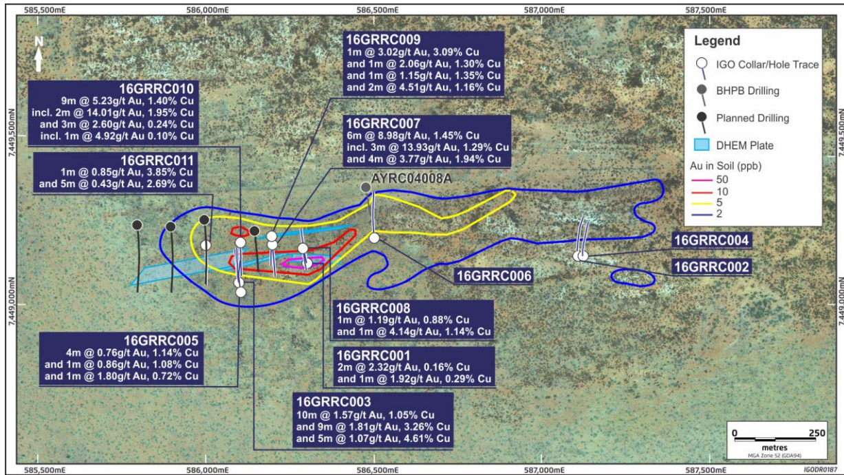
Figure 3: Grapple Prospect showing the location of the four planned drillholes, the eleven completed drill holes and the conductive plates to be tested.
