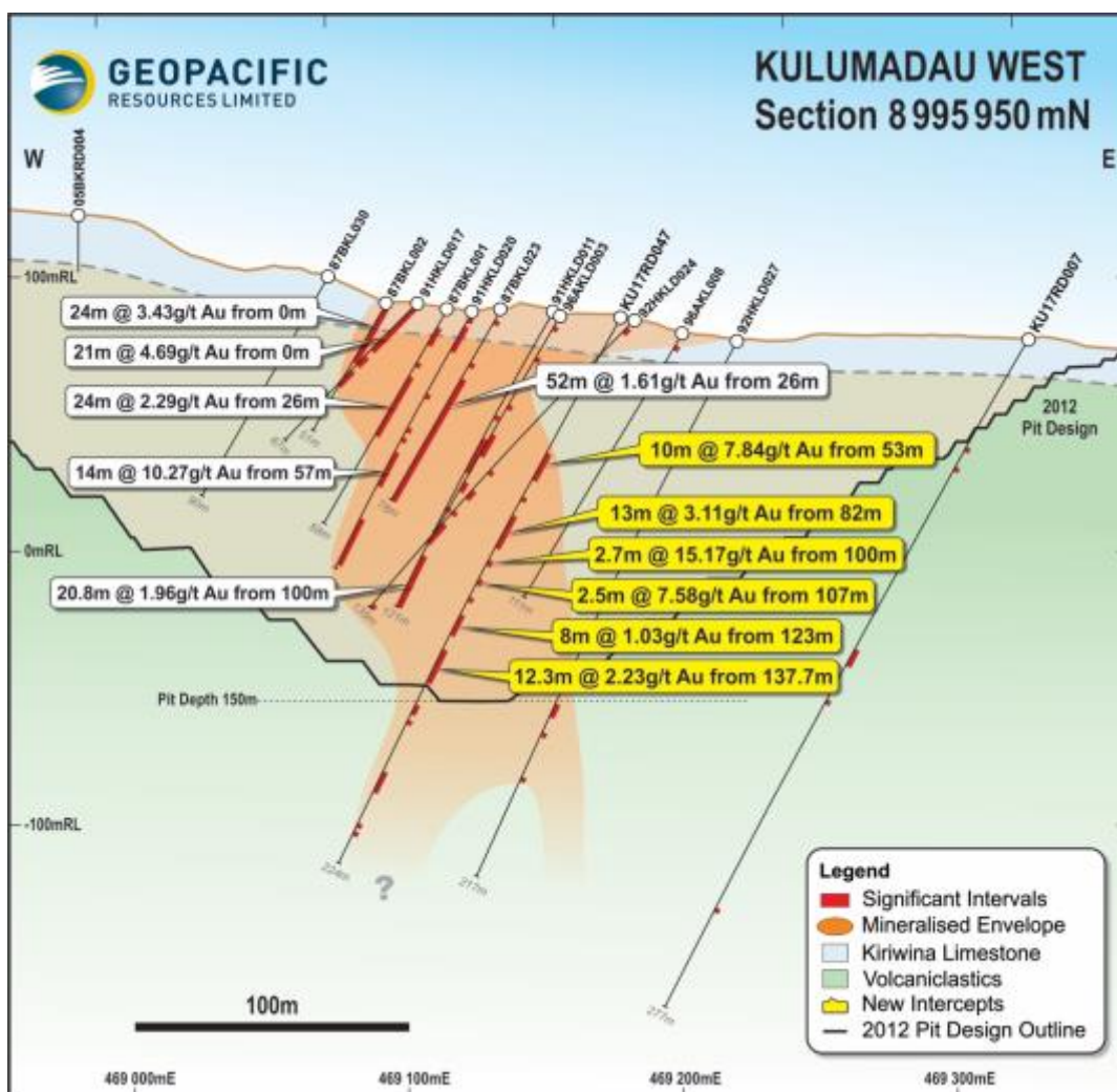
Figure : Cross section of Kulumadau West showing mineralised intersections in KU17RD047
