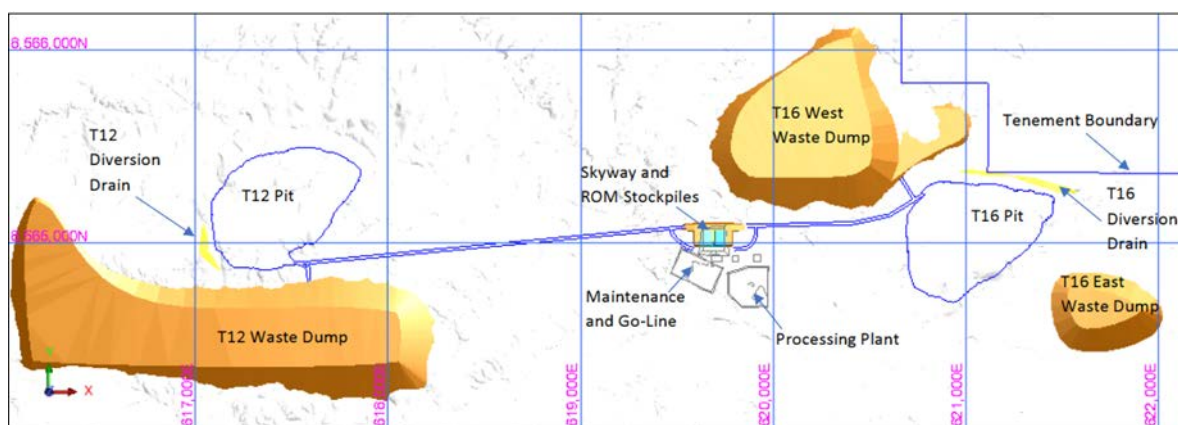
Figure 3. Mine Site Layout
