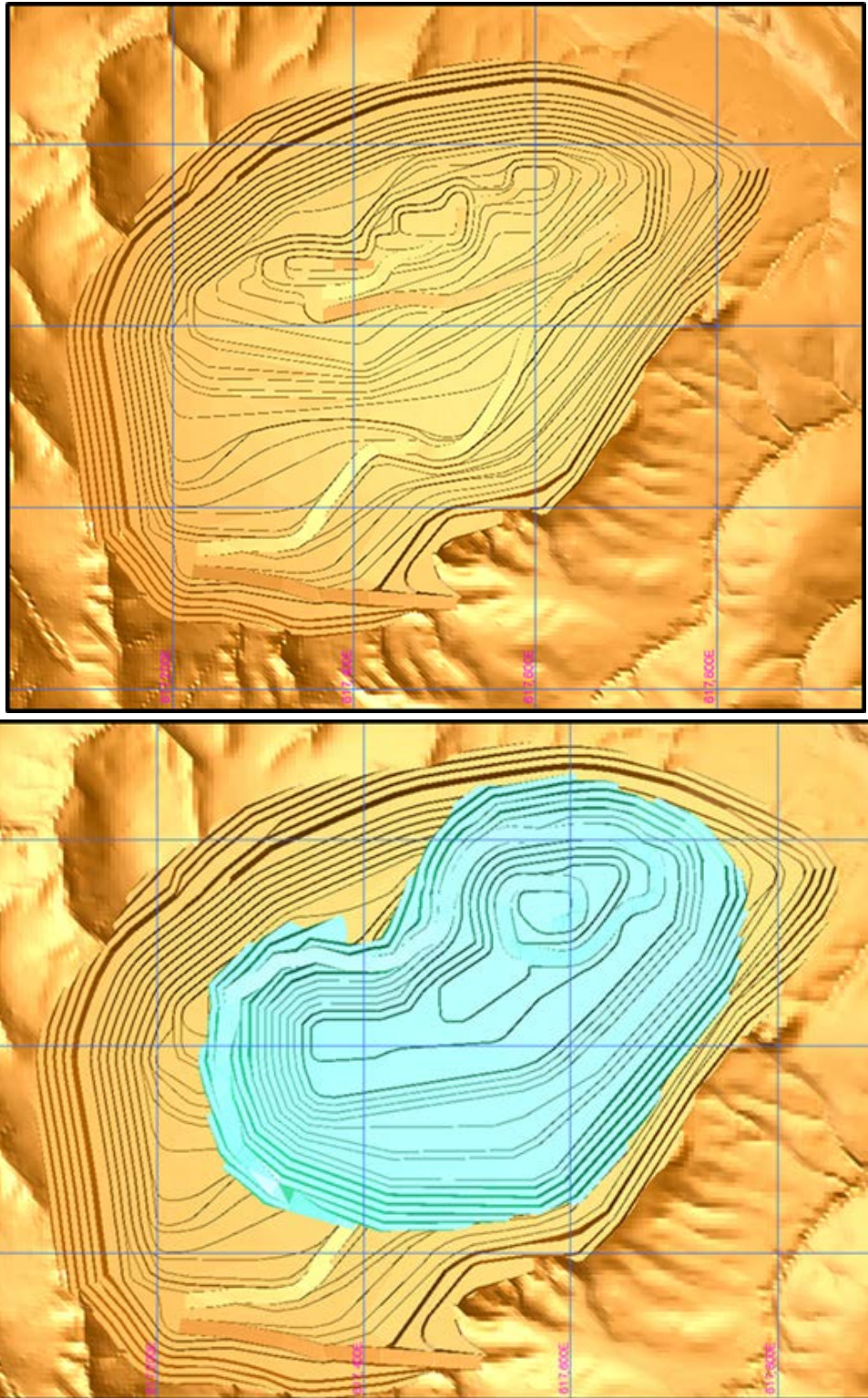
Figure 1. T12 Pit Design, showing final and starter pits
