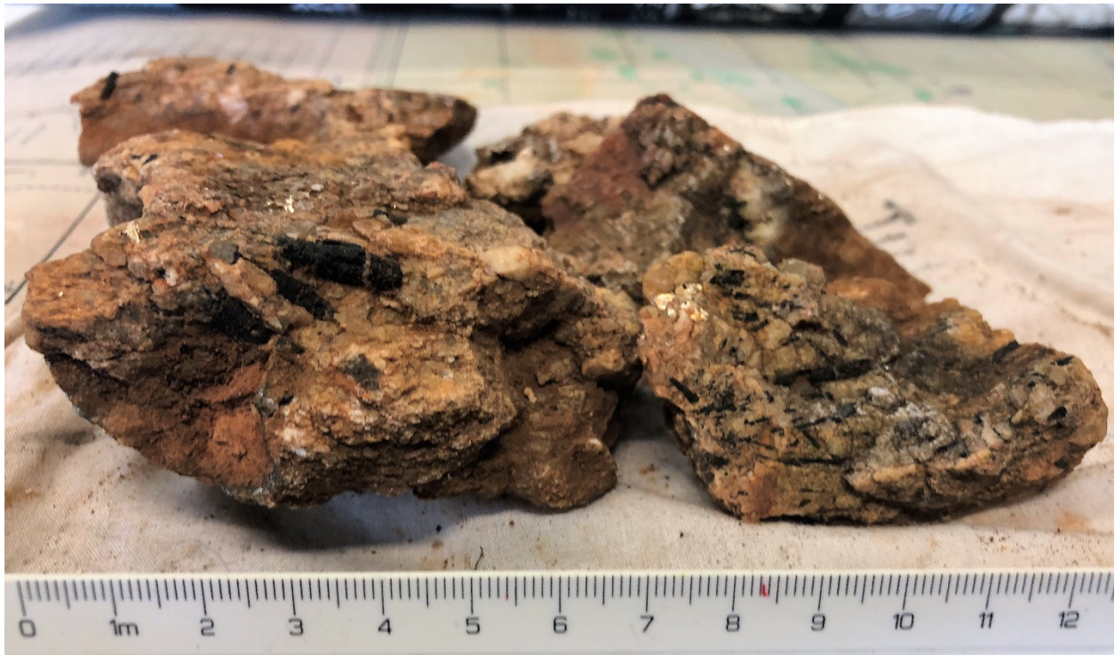
Figure 4 – Scaramucci outcrop hand specimen with “books” of mica and feldspar
