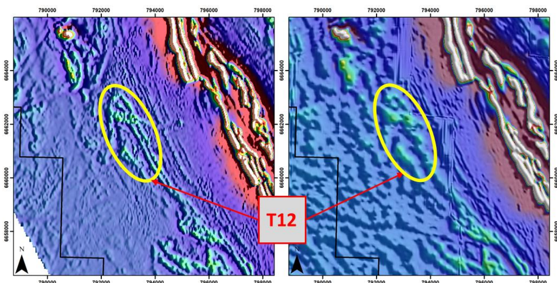
Figure 11: T12 Prospect – detailed magnetic survey (left) vs regional magnetic survey (right)
