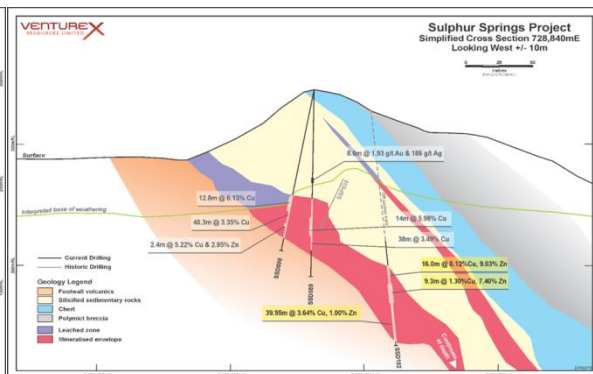
Figure 4: Sulphur Springs cross section on 728,840mE
