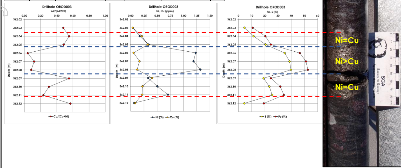
Figure A1: NITON portable XRF analysis of a profile through a massive sulphide vein hosted by country host rock gneiss. The relative metal profiles indicate fractionation between Ni and Cu to form Cu enrichment at the vein margins. This indicates that this vein is derived from the intrusion and has been injected into the gneiss.
