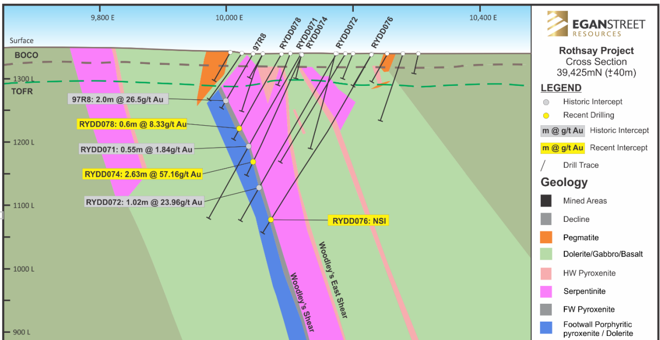
FIGURE 2 – GEOLOGICAL CROSS-SECTION SHOWING INTERSECTIONS
