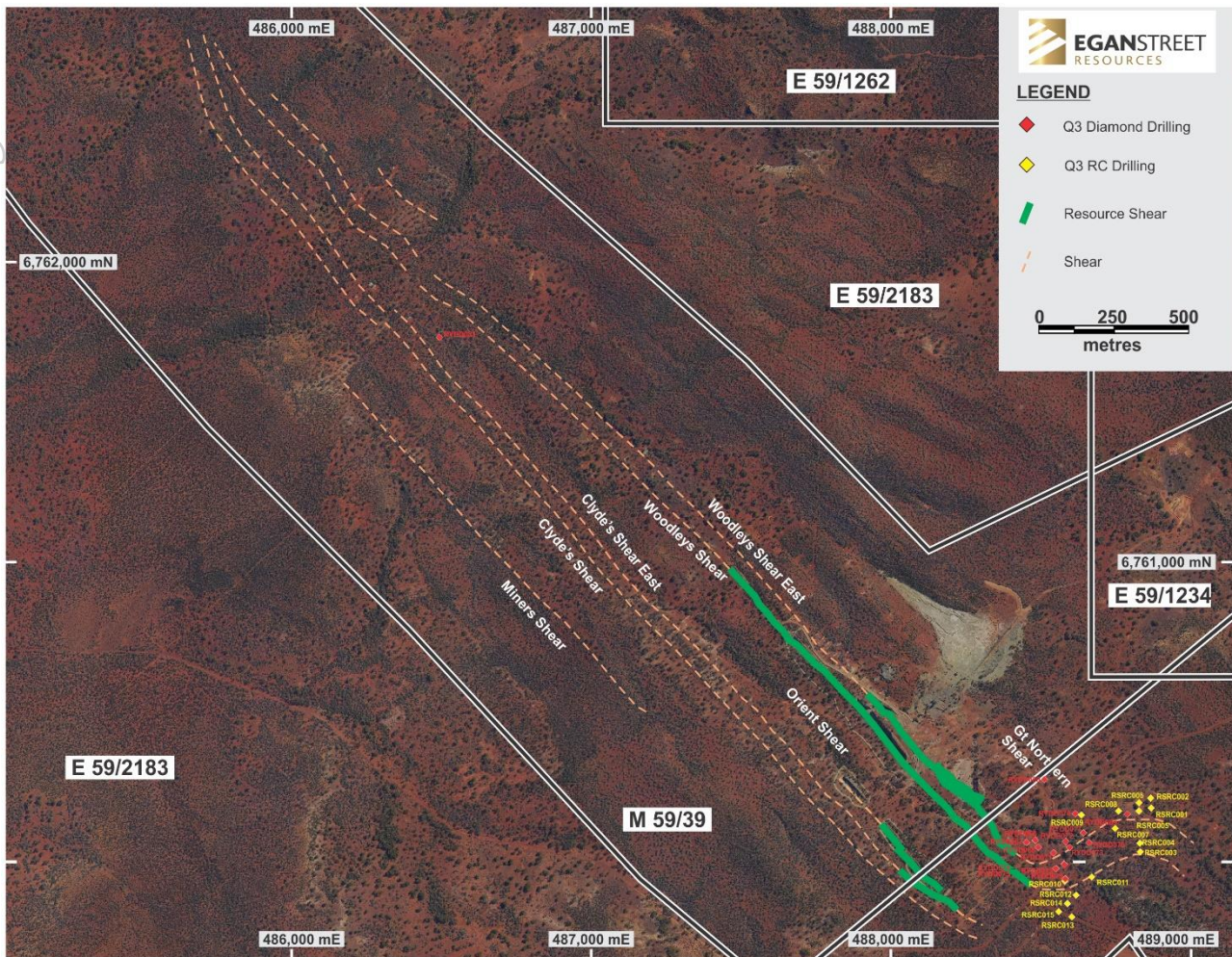
FIGURE 5 – RC AND DIAMOND DRILL COLLAR LOCATIONS
