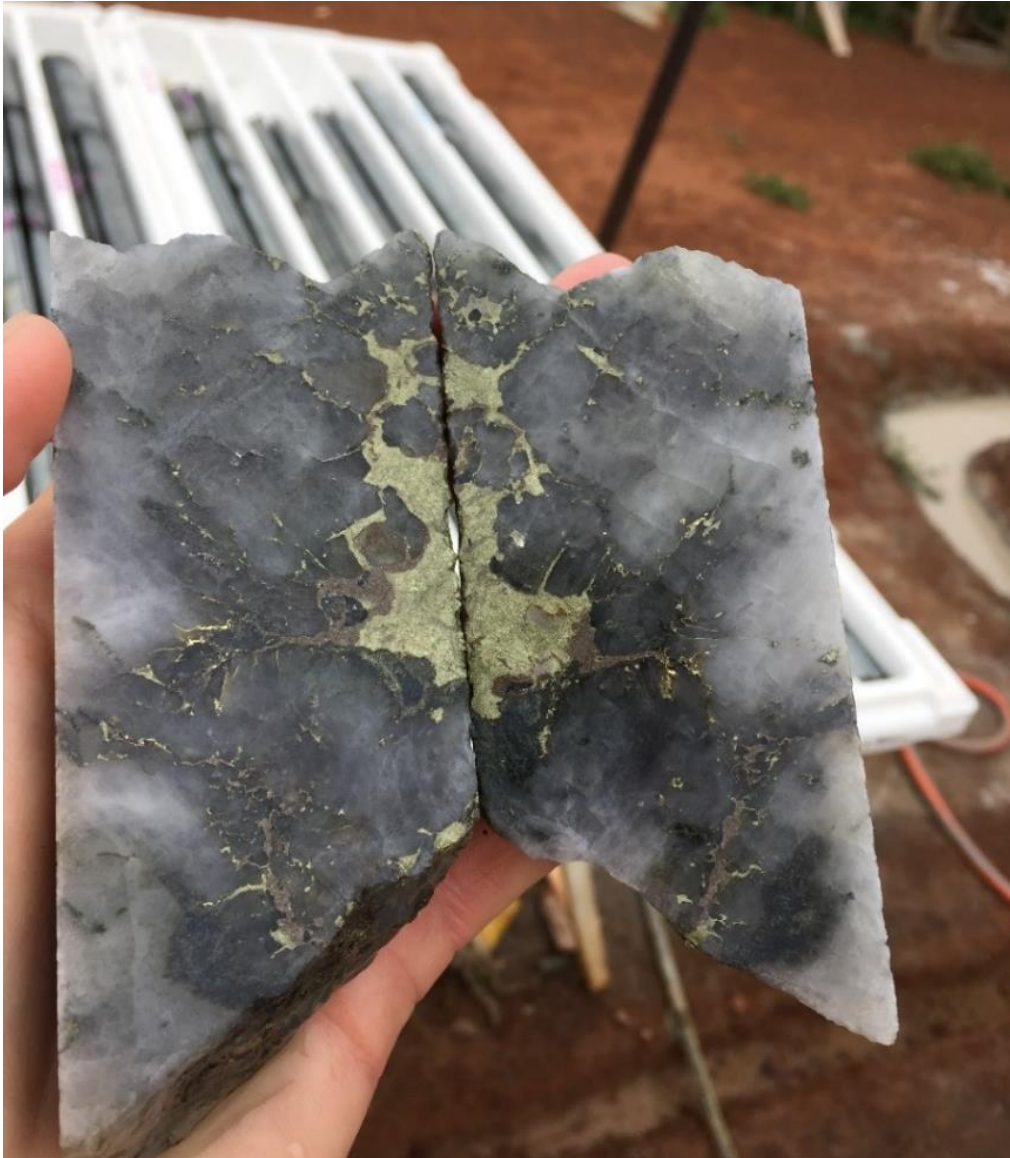
FIGURE 4 – RYDD080 DIAMOND CORE SHOWING VISABLE GOLD &amp; RETURNING 776g/t Au
