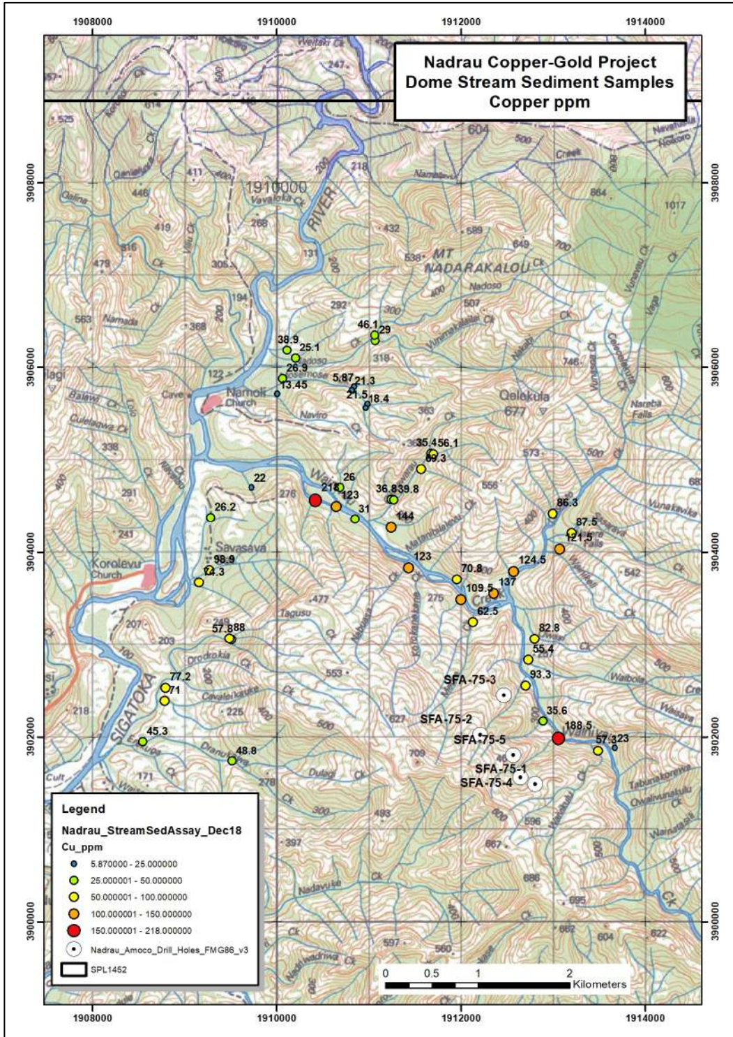
Figure 2 - Map showing the stream -sediment copper assay results from Namoli-Wainivau prospect.
