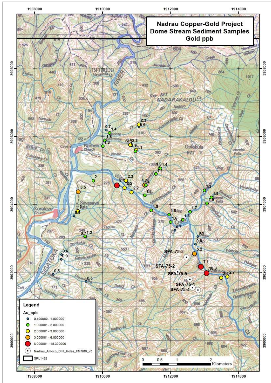
Figure 3 - Map showing the stream -sediment gold assay results from Namoli-Wainivau prospect.
