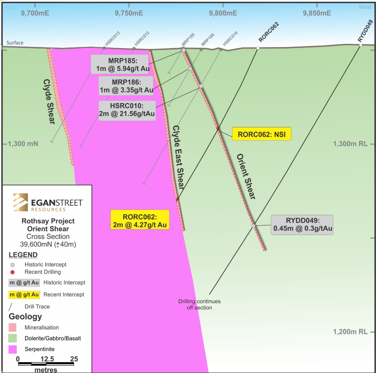
FIGURE 1 – CROSS-SECTION
