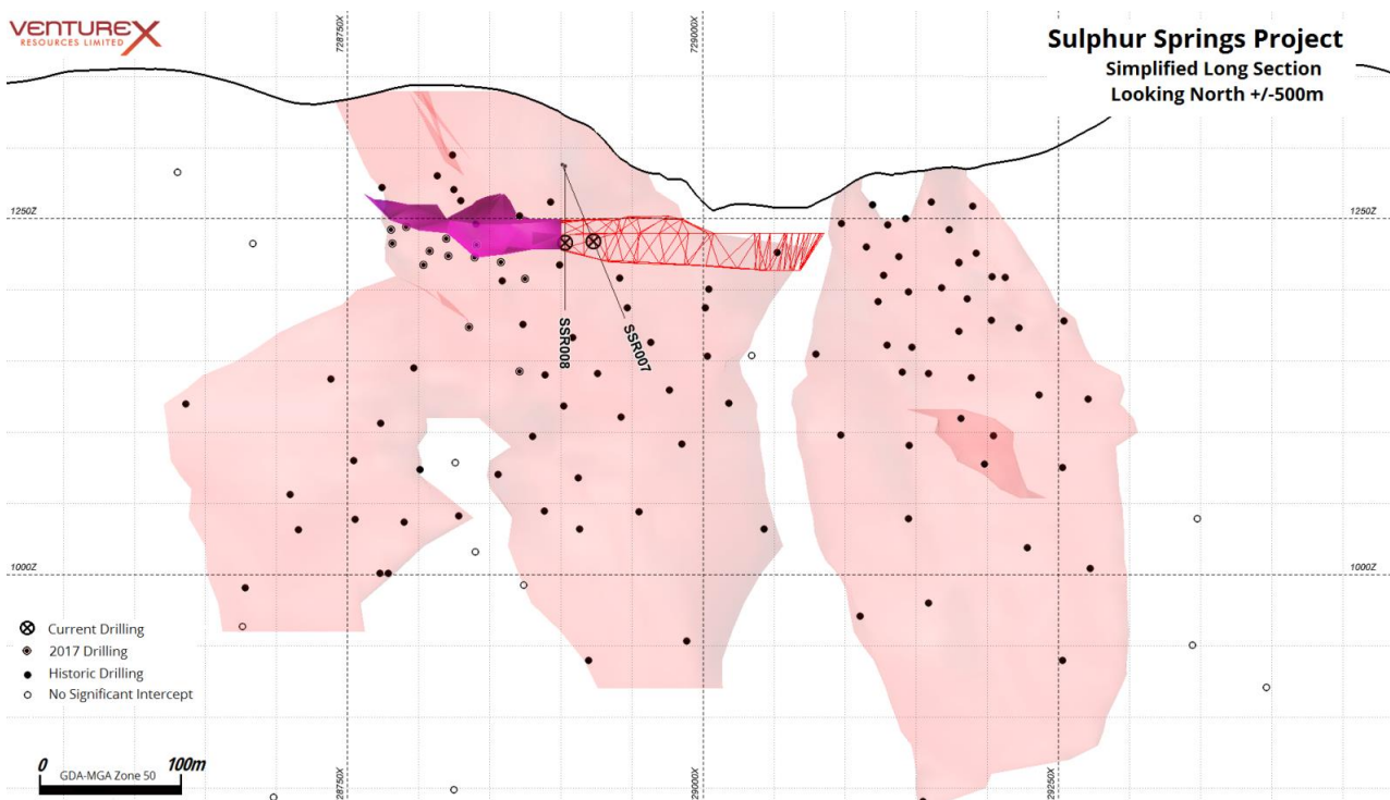
Figure 2: Sulphur Springs long-section with Inferred Supergene target zone
