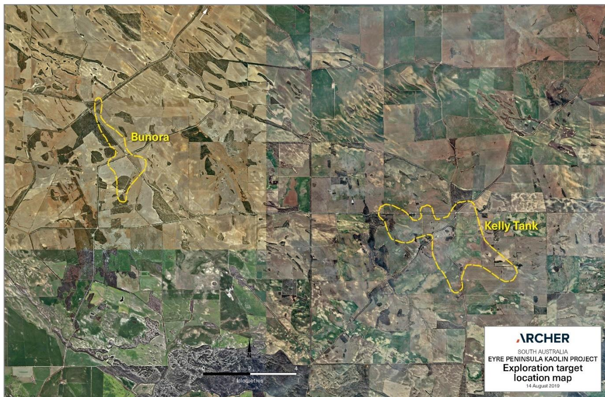
Fig. 3. EPHPA Project showing upper range areas (i.e. based on CSR exploration results) for Kelly Tank and Bunora Exploration Targets.
