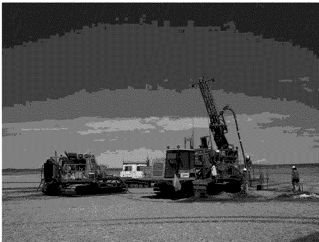
Aircore Exploration Drilling on Lake Way
