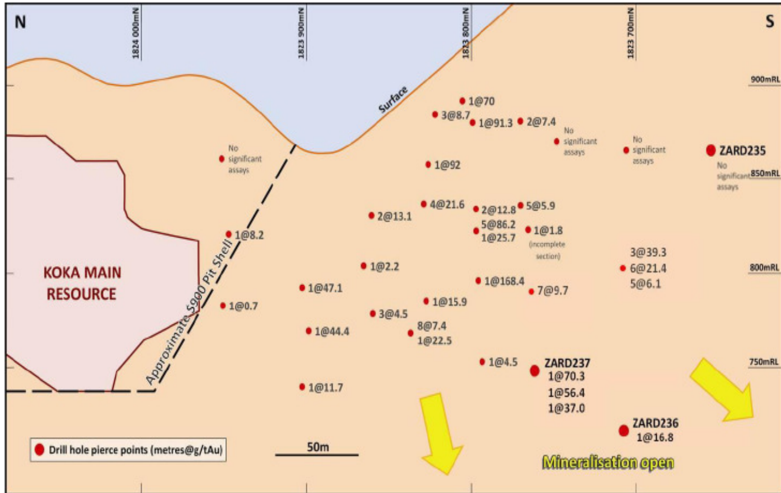
Figure 6. Koka South – schematic long section showing drillhole pierce points and main intercepts
