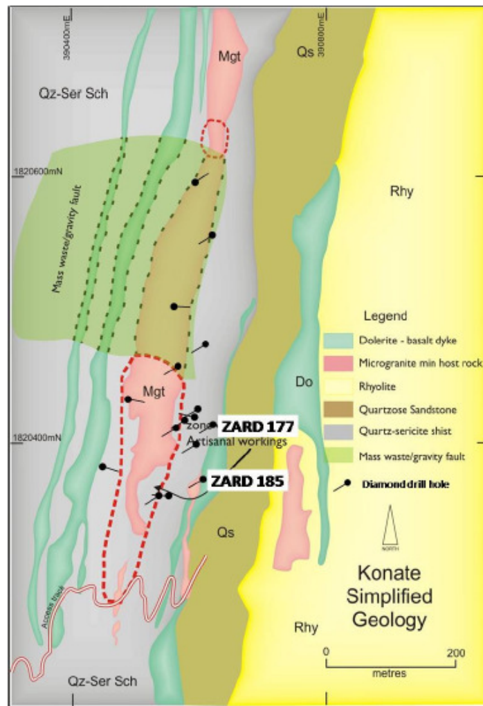
Figure 10. Konate geology and drilling
