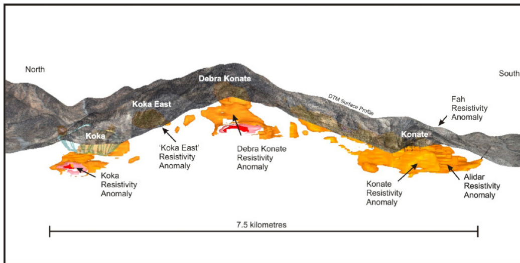
Figure 7. Long section - Koka-Konate corridor IP resistivity anomaly drill targets
