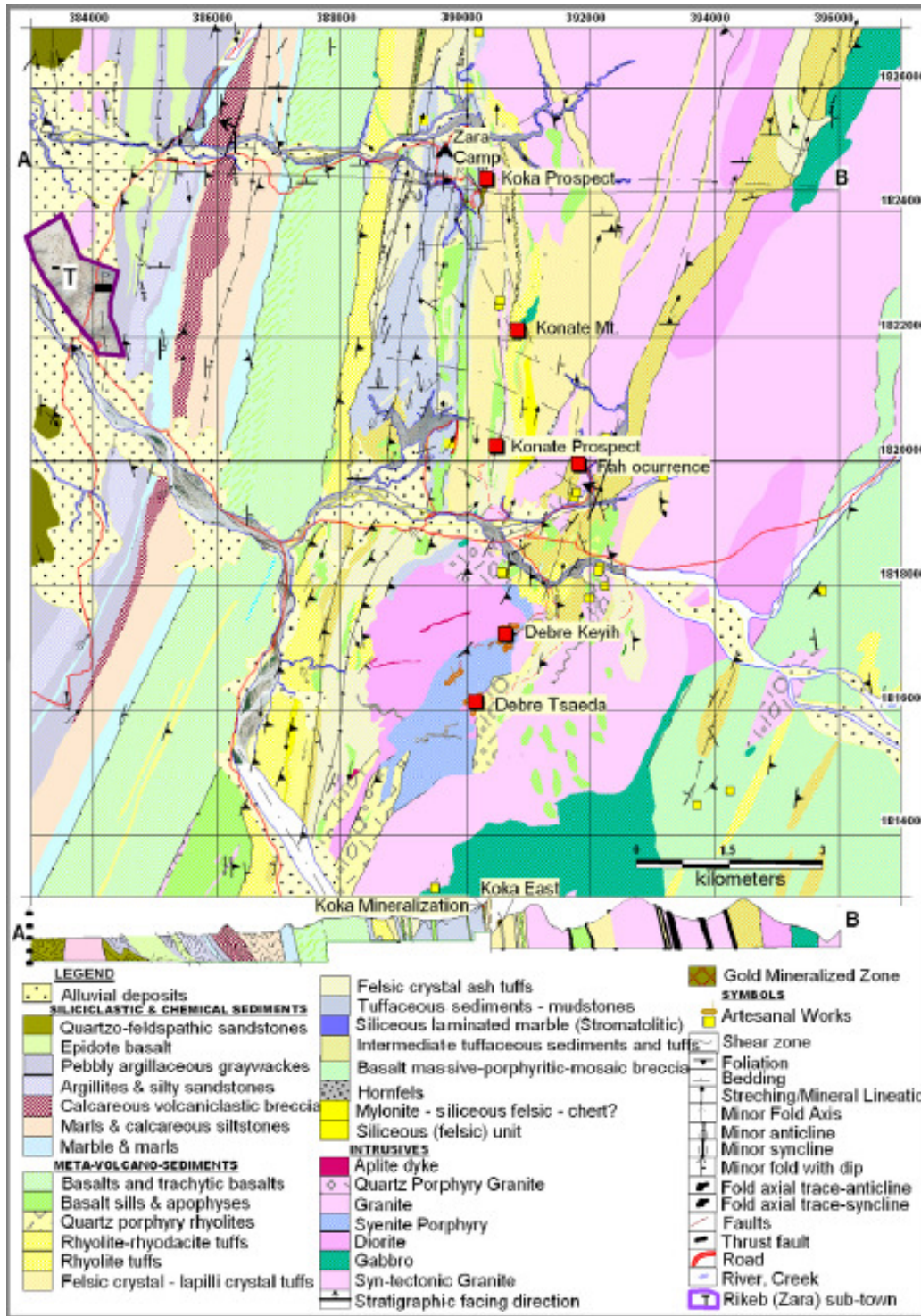
Figure 3. Regional Geology of the Zara Gold Project area
