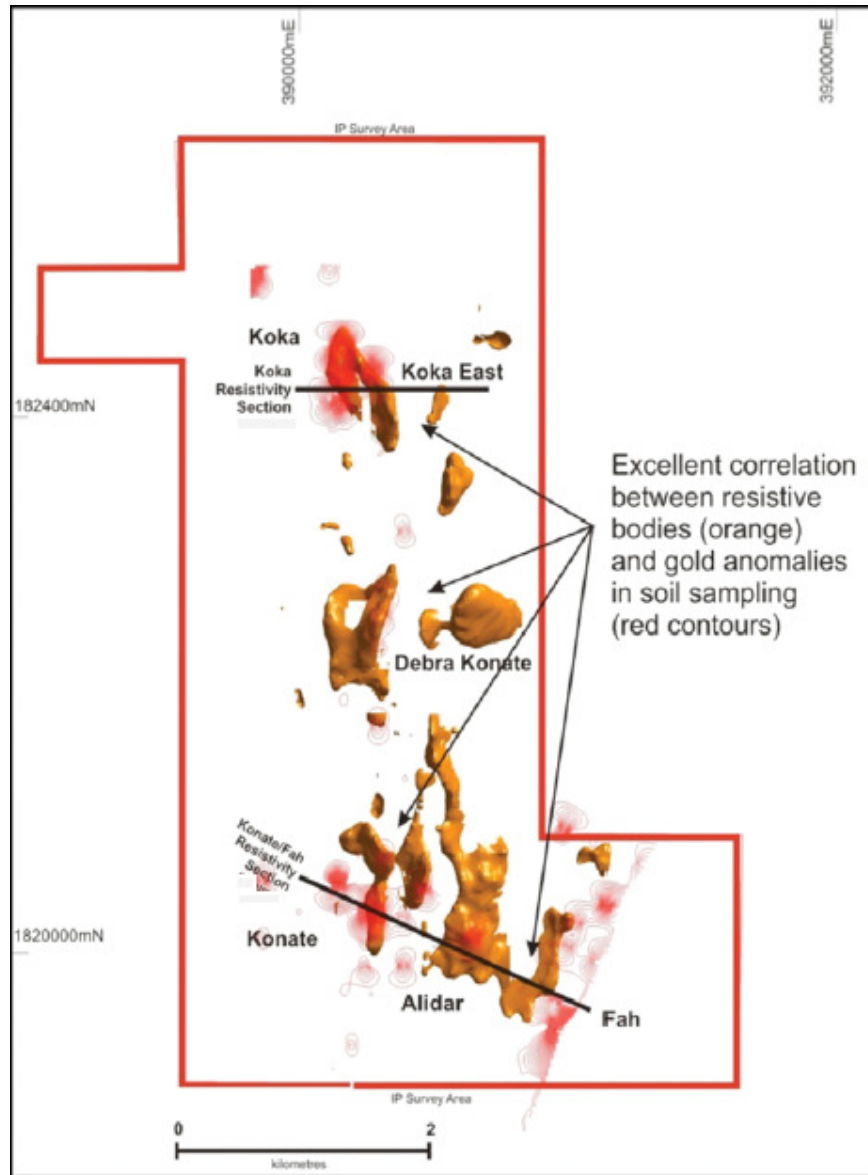
Figure 8. IP Resistivity Anomalies (brown) over gold content in soil (red contours)
