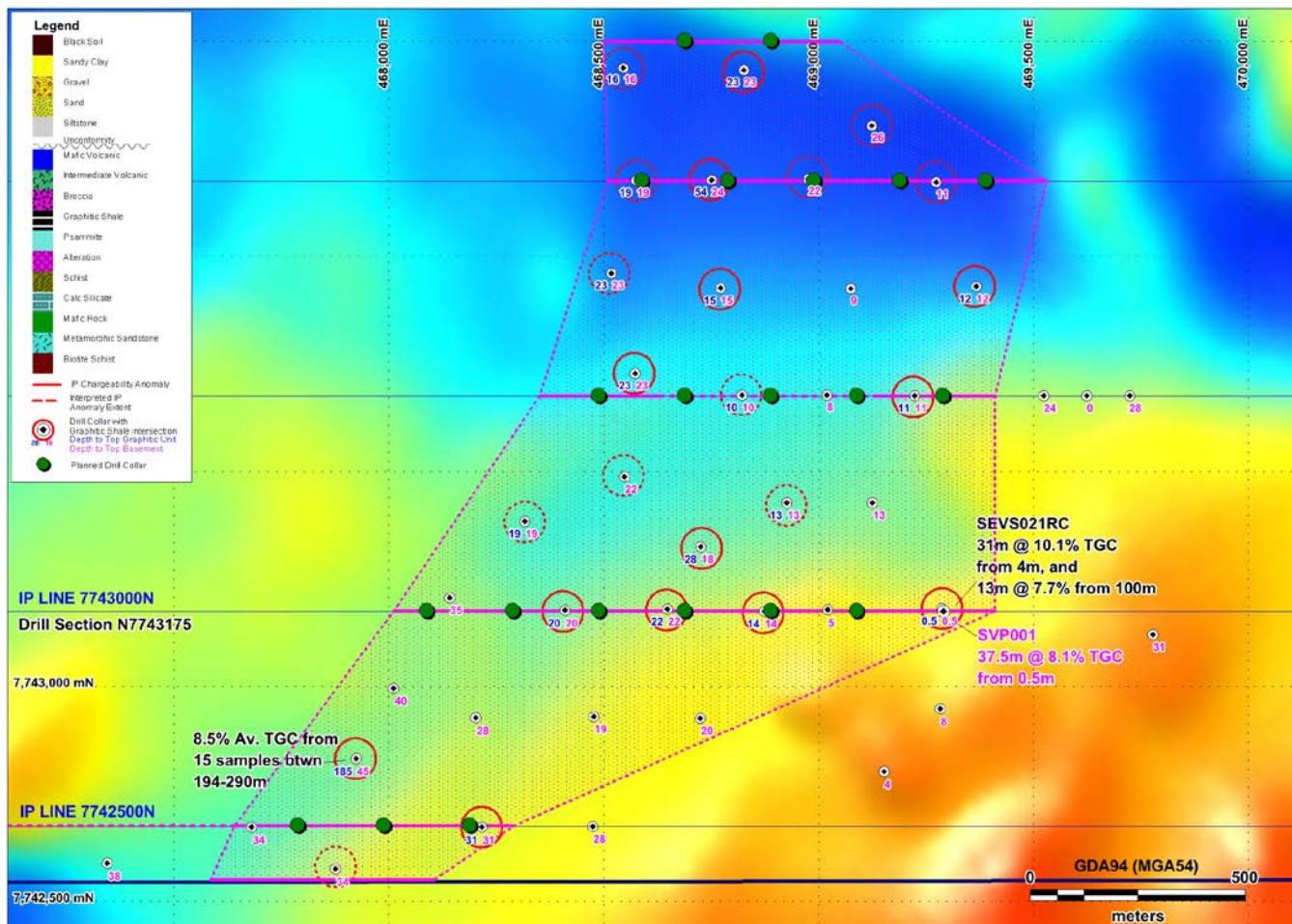
Figure 1: Sevastopol graphite target showing interpreted IP chargeability anomaly extent in plan view and planned drill collars. All historic drill collars also shown over airborne TMI TRTP magnetic image.
