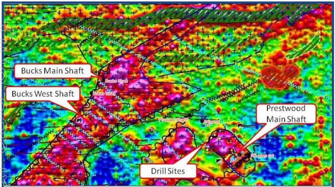
Figure 2: Geological Interpretation Projected over Magnetic Image (Analytical Signal).
