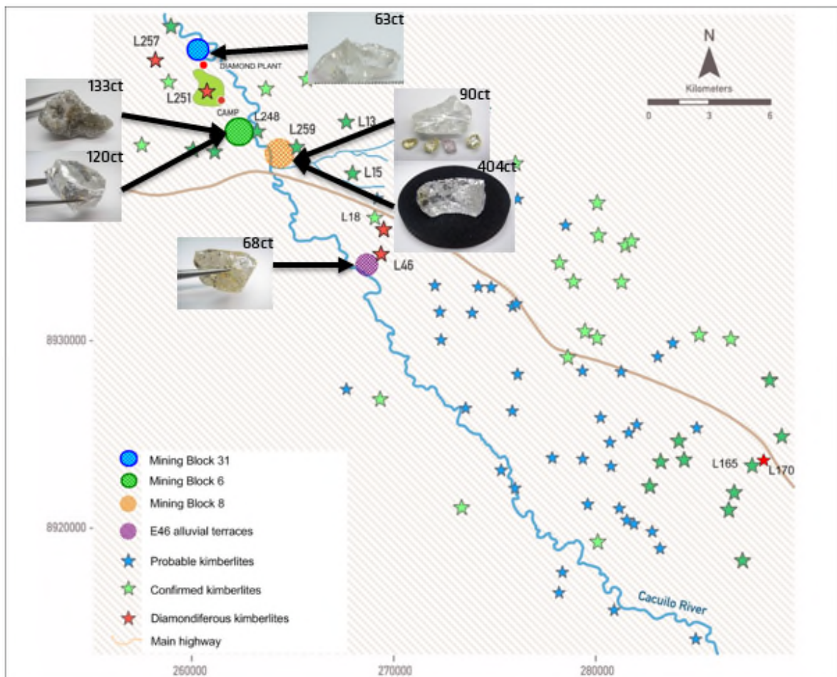
Figure 1: Location of E46 area showing the known ~20km extent of large special alluvial diamond recoveries between Mining Block 31 and E46 alluvial terraces
